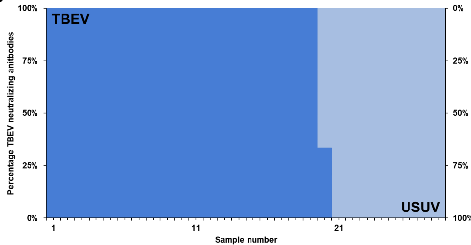
Figure S1. Bar charts depicting the percentage of neutralizing antibodies against two specific flaviviruses (WNV, TBEV, or USUV) in relation to one another for the dog (a-c) and the wild boar samples (d-f).
