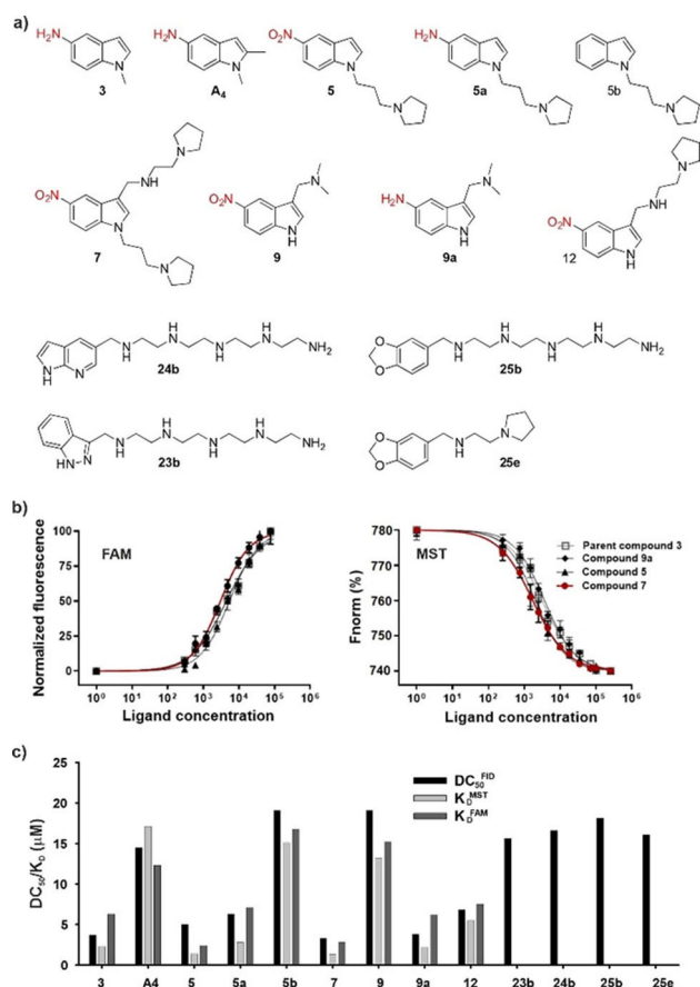
Figure 2. a) Chemical structure of best hits from initial FID experiments. b) Dose-response curves representing DC 50 and K D results from FID titrations, MST measurements and FAM experiments for compound 7 of best hits from initial FID experiments. c) DC 50 and K D results from FID titrations, MST measurements and FAM experiments. Errors are within 5%.
