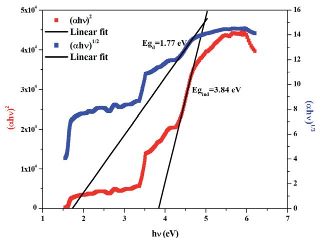
Fig. 3 Variations of (\alpha h\nu)^2 and (\alpha h\nu)^{1/2} as a function of the photon energy for the compound [\text{DMA}]_2\text{ZnCl}_4 .
