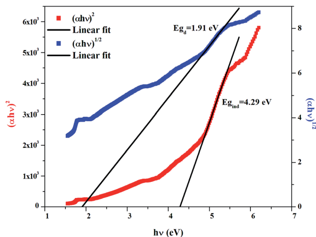
Fig. 5 Variations of (\alpha h\nu)^2 and (\alpha h\nu)^{1/2} as a function of the photon energy for the compound [\text{DMA}]_2\text{CoCl}_4 .
