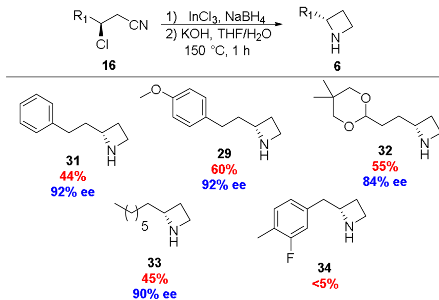
Scheme 5. Protocol for intramolecular cyclization to C2-functionalized azetidines 31–34 . 15
