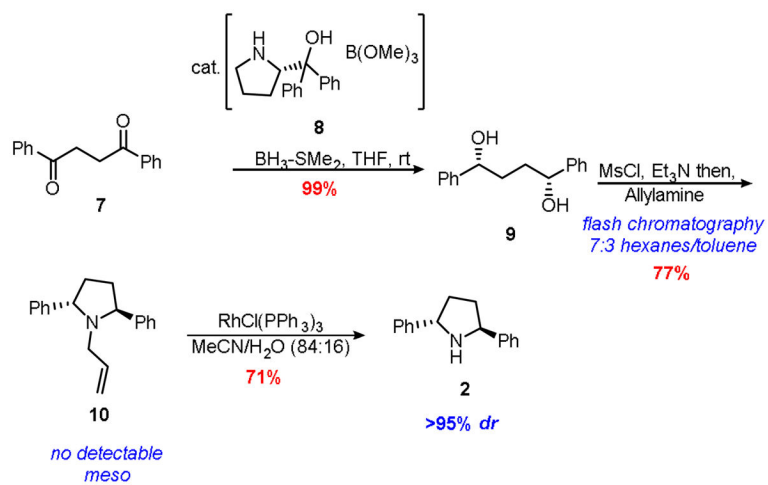
Scheme 1. Scalable, cost-effective synthesis of organocatalyst 2 .
