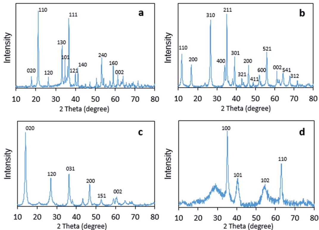
Fig. 2 Powder X-ray diffraction patterns of (a) \alpha -FeOOH, (b) \beta -FeOOH, (c) \gamma -FeOOH, and (d) \delta -FeOOH.
