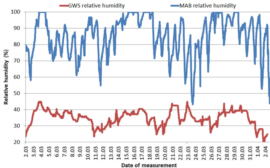
Figure 3. Ambient humidity changes during wires storage—Gdańsk welding site (GWS) and Mońki agricultural building (MAB)—1 month.
