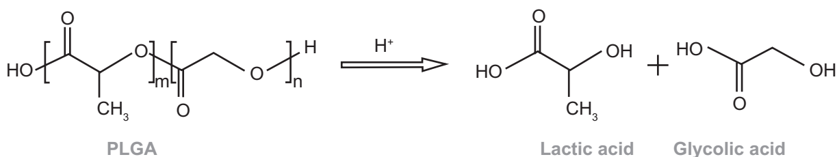
Figure 2 Degradation of polylactide-co-glycolide to lactic and glycolic acid.
