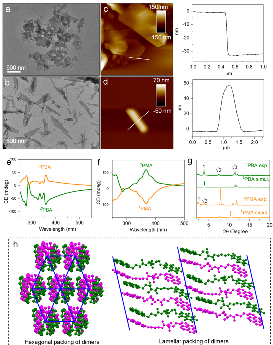
Fig. 7 Self-assemblies. (a and b) TEM images of self-assembled L -PMA and L -PBA in a mixture of \text{CHCl}_3/\text{MCH} (2/8 by volume, 1 mM); (c and d) the corresponding AFM images and cross-section profiles ( 3 \times 3 \mu\text{m} and 5 \times 5 \mu\text{m} , respectively); (e and f) CD spectra of self-assemblies. (g) XRD pattern comparison between simulated powder patterns and experimental results; (h) hexagonal and lamellar packing of dimers of L -PMA and L -PBA, respectively.
