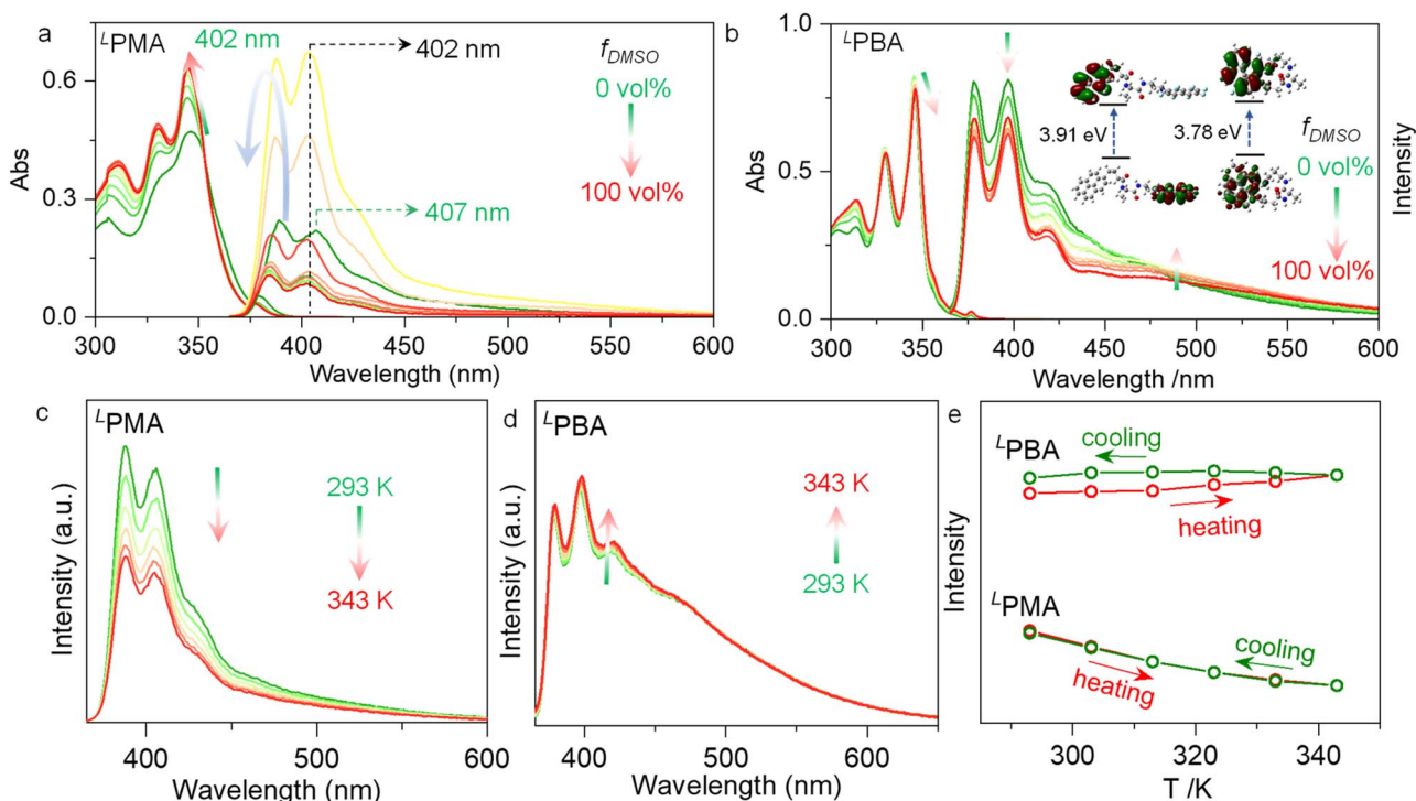
Fig. 3 (a) Absorption and emission spectra of L PMA (0.2 mM) with different volume fractions of DMSO ( f_{\text{DMSO}} ) against CHCl 3 . (b) Absorption and emission spectra of L PBA (0.2 mM) with different volume fractions of DMSO ( f_{\text{DMSO}} ) against CHCl 3 . The inset shows the HOMO–LUMO gap of the free monomer and folded L PBA. Temperature-variable emission spectra of (c) L PMA and (d) L PBA in DCE (0.2 mM), as well as (e) the summarized max. intensity as a function of temperature.
