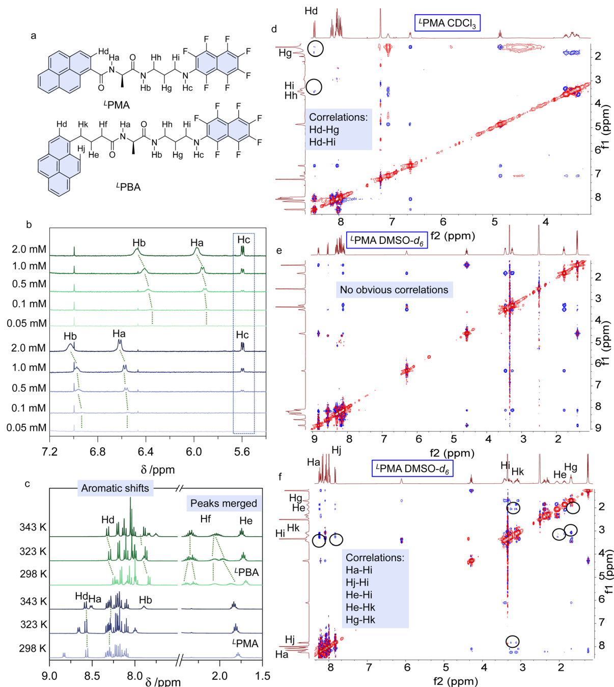
Fig. 4 1 H NMR studies. (a) Proton assignments of L PMA and L PBA. (b) Concentration-dependent 1 H NMR spectra of L PMA and L PBA in CDCl 3 . (c) Temperature-variable 1 H NMR spectra of L PMA and L PBA in DMSO- d 6 (10 mM). (d–f) 2D NOESY spectra of L PMA and L PBA in CDCl 3 (saturated) and DMSO- d 6 (10 mM).
