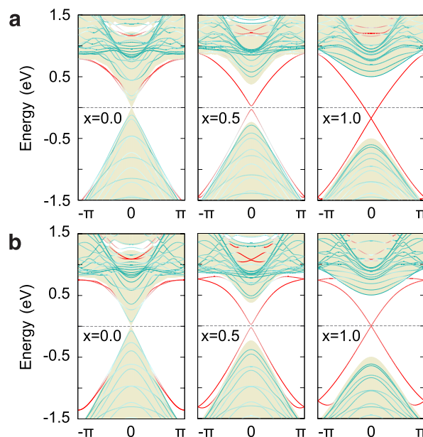
Figure 5 | Edge states of armchair-edged Bismuthane nanoribbons. A similar plot as in Fig. 4 with the SOC strength ( x ) set to 0, 50 (0.5), and to 100% (1.0) of the true value. The armchair-edged bismuthane nanoribbons have a linear dispersion with the Dirac point at \Gamma regardless of the edge passivation; (a) no passivation and (b) the hydrogen passivation. The 2D bulk-bands projected on the 1D Brillouin zone are depicted in green.
