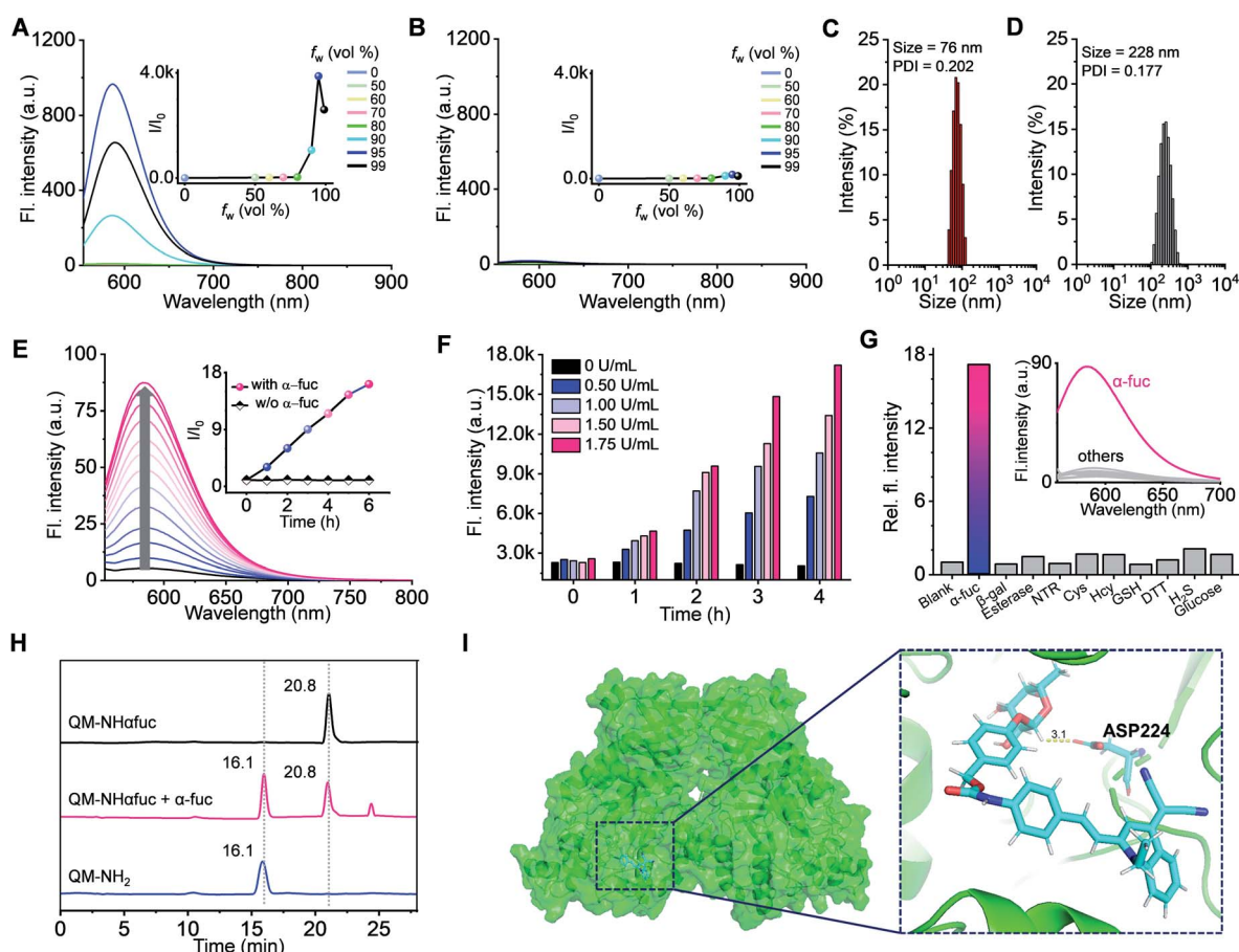
Fig. 4 Evaluation of QM-NH \alpha fuc as an \alpha -fuc-responsive AIE fluorescence probe. Emission spectra ( \lambda_{\text{ex}} : 543 nm) of (A) QM-NH _2 (10 \mu\text{M} ) and (B) QM-NH \alpha fuc (10 \mu\text{M} ) in a mixture of THF with different aqueous fractions ( f_w ). Inset: plots of relative fluorescence intensity at 586 nm against f_w . DLS data for (C) QM-NH _2 (5 \mu\text{M} ) and (D) QM-NH \alpha fuc (5 \mu\text{M} ) in pure water. (E) Time-dependent emission spectra ( \lambda_{\text{ex}} : 543 nm) of QM-NH \alpha fuc (20 \mu\text{M} ) recorded in the presence of \alpha -fuc (2 U mL -1 ). Inset: plots of the relative intensity at 586 nm as a function of time. (F) Fluorescence intensity of QM-NH \alpha fuc in the presence of different concentration of \alpha -fuc recorded as a function of time. (G) Fluorescence response of QM-NH \alpha fuc (20 \mu\text{M} ) after 6 h incubation with \alpha -fuc or other analytes. (H) HPLC monitoring of the hydrolysis of QM-NH \alpha fuc seen in the presence of \alpha -fuc. (I) Proposed binding mode for QM-NH \alpha fuc within the active site of \alpha -fuc.
