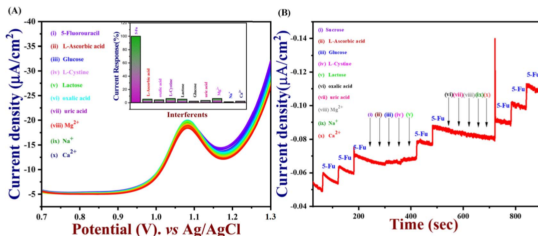
Fig. 7 (A) Selectivity of the PTh/h-BN/GCE with the addition of the same concentration of the interference molecules by DPV techniques (inset: histogram of current response vs. various interferent ions), (B) selectivity of the PTh/h-BN/GCE with the addition of the same concentration of the interference molecules by the amperometry technique.
