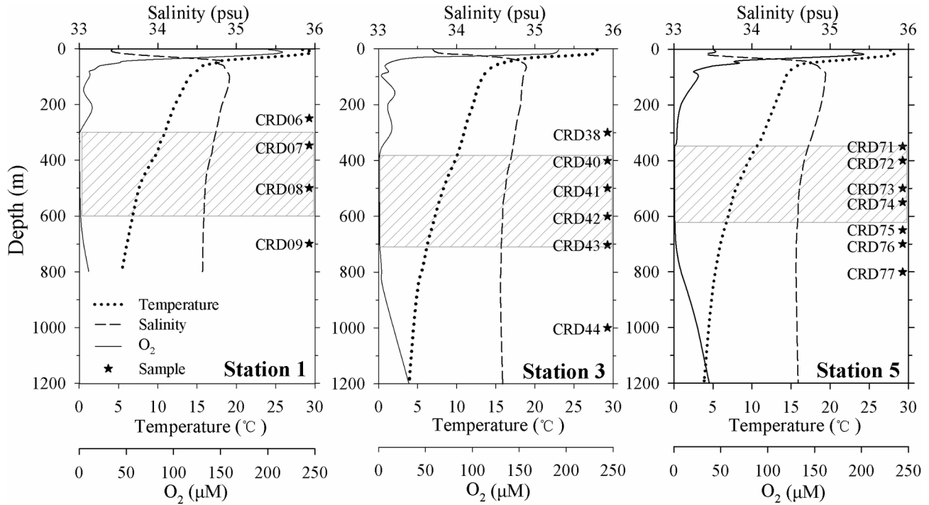
Figure 2. Hydrographic conditions of the sampling stations. Shadow layers indicate the core of the oxygen minimum zones (OMZs) characterized by dissolved oxygen concentration lower than 1.0 µM.
