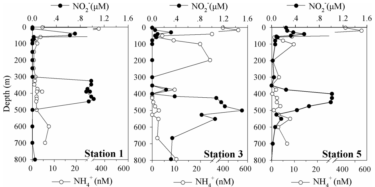
Figure 3. Vertical distributions of nitrite (NO 2 - ) and ammonium (NH 4 + ) in the water columns of the sampling stations in Costa Rica Dome (CRD).
