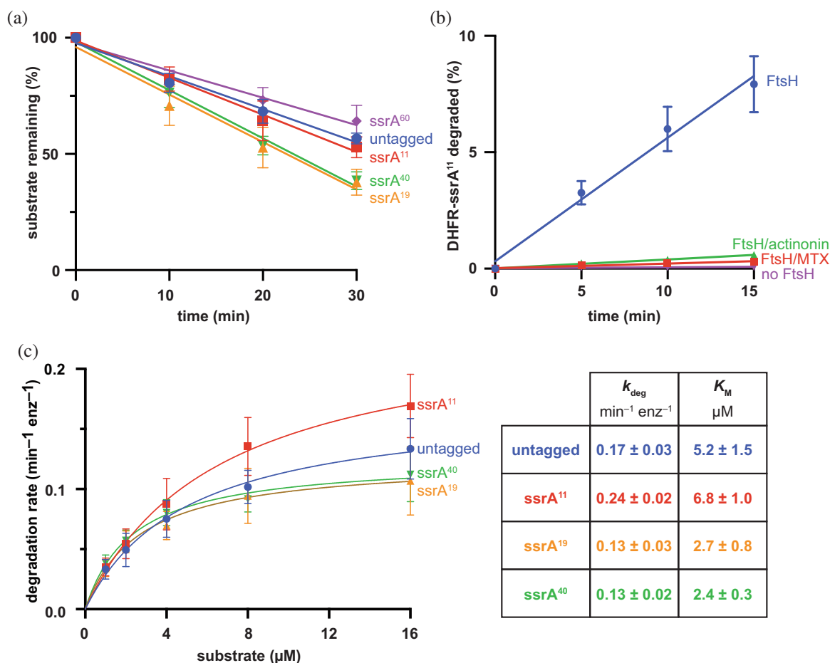
FIGURE 3 FtsH degradation of DHFR constructs. (a) Rates of FtsH 6 (1 \mu\text{M} ) degradation of untagged DHFR or different DHFR-ssrA tail variants (5 \mu\text{M} each) at 42°C. Values are means ( n \geq 3 ) \pm 1 SD, and lines are linear least square fits. (b) Fluorophore-labeled DHFR-ssrA 11 (16 \mu\text{M} ) was incubated with FtsH 6 (0.5 \mu\text{M} ), ATP, and a creatine-kinase regeneration mix at 37°C, and degradation kinetics were monitored by measuring the fluorescence of acid-soluble peptides released. Experiments are also shown in the presence of the actinonin inhibitor (10 \mu\text{M} ), methotrexate (125 \mu\text{M} ), or the absence of FtsH. (c) (Left) Rates of FtsH 6 degradation of different concentrations of untagged DHFR or DHFR-ssrA tail variants at 37°C. Values are means ( n \geq 3 ) \pm 1 SD. Lines are nonlinear least squares fit to the Michaelis-Menten equation. (Right) Average k_{\text{deg}} and K_M values \pm 1 SD from three or four independent experiments
