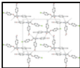
Fig. 2. The crystal packing and C-H...O hydrogen-bond interactions (dashed lines) of the title compound viewed down the a axis.
