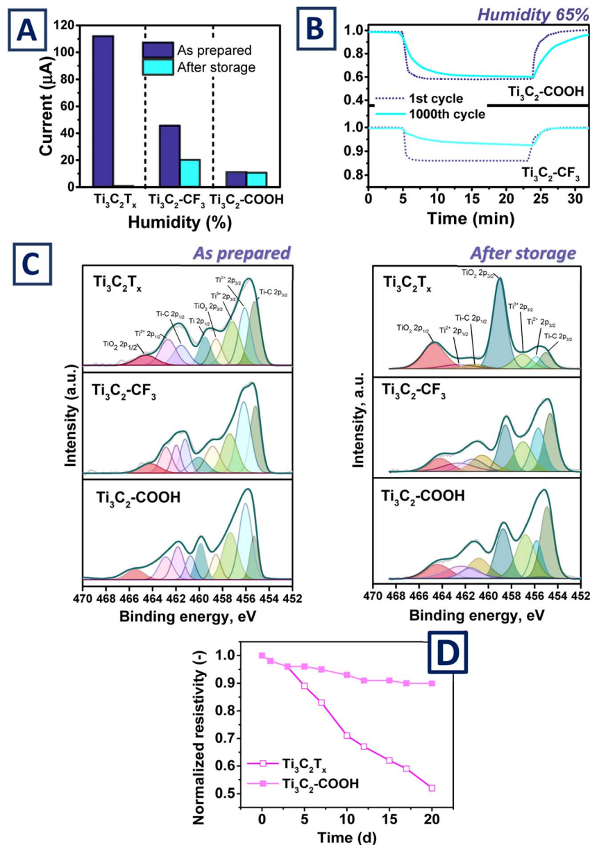
Fig. 5 (A) Conductance of pristine and grafted ( i.e. , protected) Ti 3 C 2 T x films measured immediately after film deposition and after storage for 6 months at ambient conditions; (B) changes of grafted Ti 3 C 2 T x films response to humidity presence induced by flakes storage; (C) deconvolution of characteristic Ti 2p XPS peak, measured before and after storage of pristine and grafted Ti 3 C 2 T x thin films. (D) Estimation of sensor stability under operation conditions.
