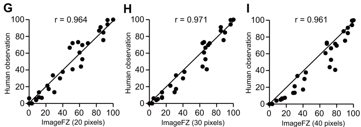
Figure 5. The freezing percentages calculated from the images at different freezing criterion values using ImageFZ and those measured through human observations were compared. The fear conditioning tests were conducted using male C57BL/6J mice ( n=5 ). During the tests, two observers recorded the freezing behavior, and the live images were captured using the ImageFZ program. The freezing percentages in each 60 sec bin were calculated from the images (1 frame/sec) through ImageFZ offline analysis, setting the parameter values of 'Freezing criterion (pixels)' to 20, 30, or 40 pixels. Each dot represents a freezing percentage of each 60-sec bin. Pearson's correlation coefficients between the data obtained from human observation and the ImageFZ analysis were calculated in each test. Click here to view larger image.
