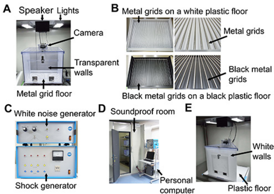
Figure 1. Apparatuses for the contextual and cued fear conditioning test. (A) An acrylic square chamber for the conditioning and context test, (B) metal grids on a white plastic floor for black, agouti, or dilute brown mice (top) and electrifiable black metal grids on a black plastic floor for white mice (bottom); enlarged images of the grids are shown in the right panel, (C) a white noise/tone generator and a shock generator, (D) a soundproof room, and (E) an acrylic triangular chamber with a flat floor for the cued test. Click here to view larger image.
