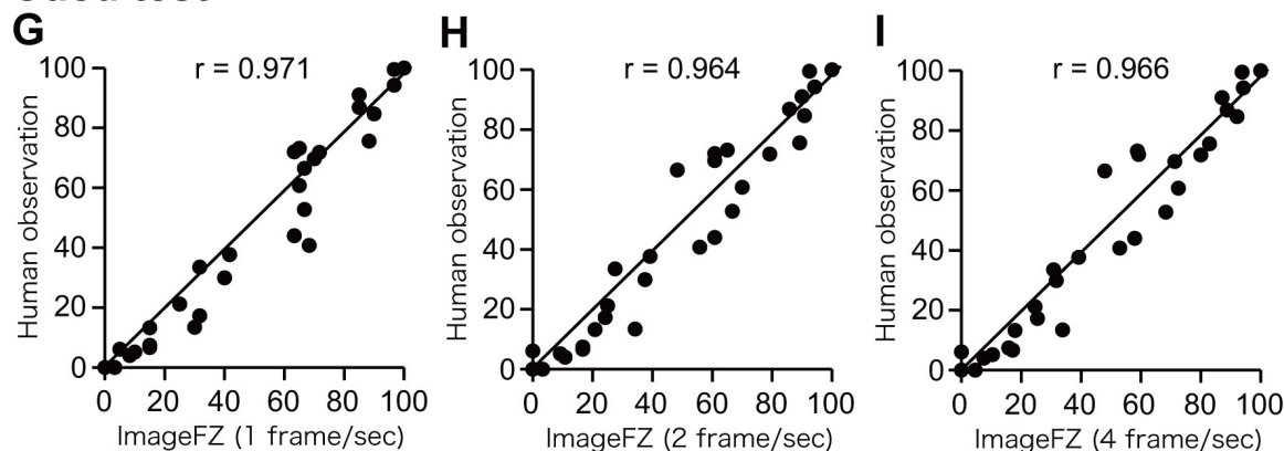
Figure 4. Comparisons of the freezing percentages calculated from images at different frame rates using ImageFZ with those measured through human observation. The fear conditioning tests were conducted using male C57BL/6J mice ( n=5 ). During the tests, two observers scored the freezing behavior. Simultaneously, live images were captured at 4 fps using the ImageFZ program. The files captured at 4 fps were downsized after extracting the frames to correspond to images captured at 1 fps or 2 fps. The parameter values of 'Rate (frame/sec)' were set to 1, 2, or 4 fps, and freezing percentages in each 60-sec bin were calculated from image files using ImageFZ offline analysis. Each dot represents a freezing percentage of each 60-sec bin. Pearson's correlation coefficients between the data obtained from human observation and ImageFZ analysis were calculated. Click here to view larger image.
