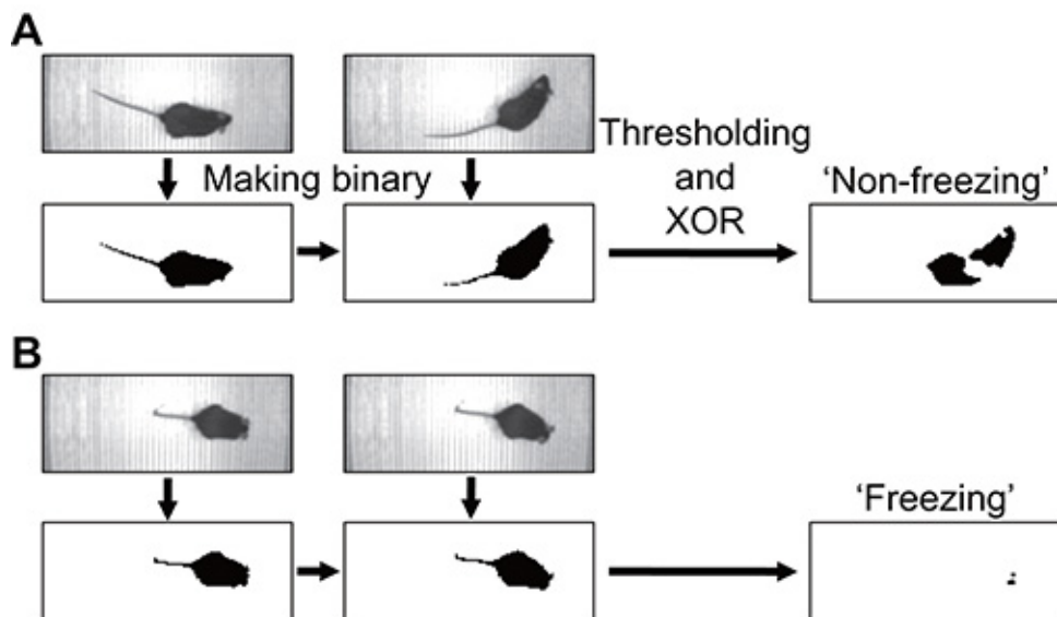
Figure 3. Image analysis by the ImageFZ software program. For each pair of successive images, the amount of area (pixels) through which the mouse moved is calculated by ImageFZ. When this area is below a certain threshold (e.g. 30 pixels), the behavior is judged to be 'freezing'. When the amount of area equals or exceeds the threshold, the behavior is considered to be 'non-freezing'. Click here to view larger image.
