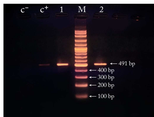
Fig .2. Gel-Electrophoresis of the PCR products of integrons by hep primers (I lanes) and control samples (positive control: C+, negative control: C-).
