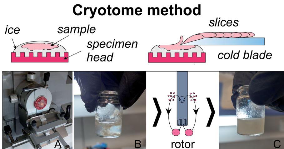
Fig. 1 Homogenization with the use of a microtome-cryostat: (A) slicing of a mounted on ice tissue; (B) collecting slices into a vial with addition of cold MeOH; (C) the sample after 10 s of homogenization with rotor homogenizer.
