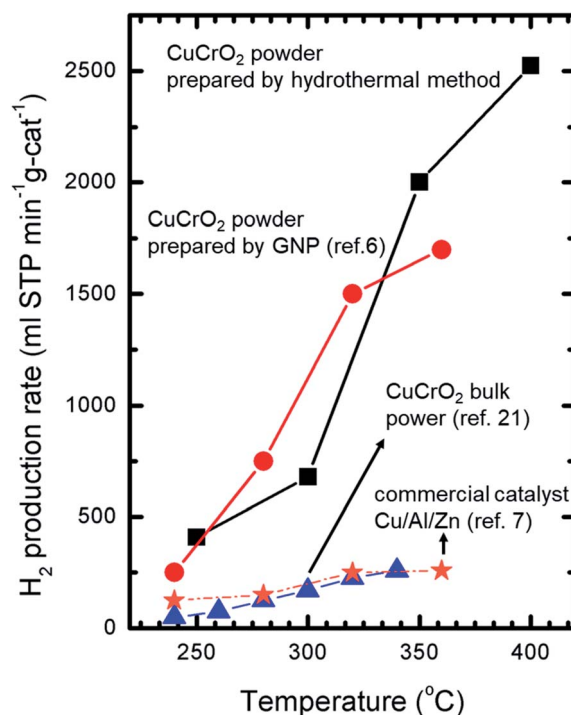
Fig. 6 The \text{H}_2 production rate versus reaction temperatures in the SRM process.
