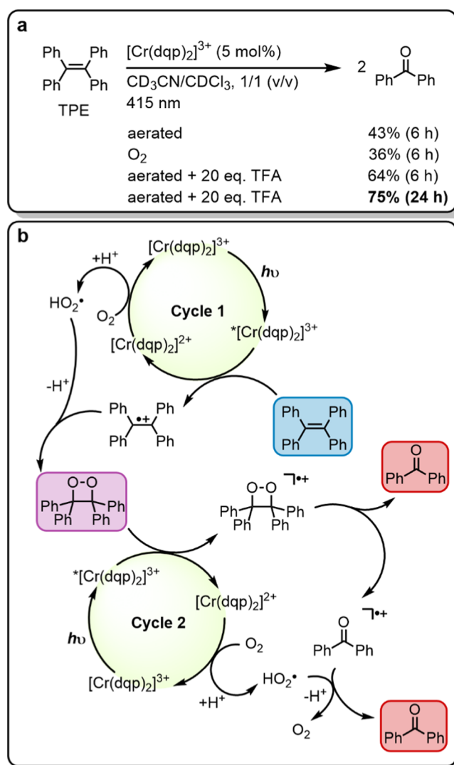
Figure 7. (a) Photocatalytic oxygenation of 1,1,2,2-tetraphenylethene (TPE) with oxygen followed by C–C bond cleavage to two benzophenone units. Irradiation with a 415 nm LED (7.0 W output) with 400 nm long pass filter, 15 mM substrate, 2.0 equiv of 1,4-dichlorobenzene as internal ^1\text{H} NMR standard, 20 equiv of trifluoroacetic acid (TFA), and 5 mol % of catalyst in 0.6 mL of \text{CD}_3\text{CN}/\text{CDCl}_3 (1/1, v/v) in closed NMR tubes under air at up to 35 °C (temperature fluctuations caused by the LED radiation). Yields are referenced to the internal standard. (b) Plausible mechanism based on a previous report with 9-mesityl-10-methylacridinium ion ( \text{Acr}^+\text{-Mes} ) as a photocatalyst. 72
