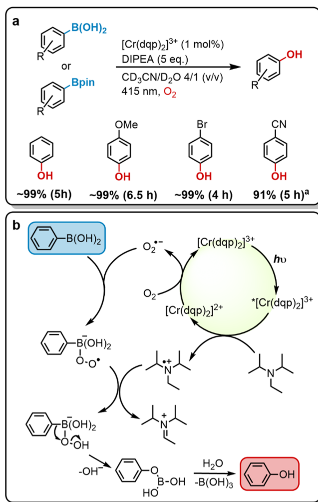
Figure 8. (a) Photocatalytic aerobic oxidative hydroxylation of arylboronic acids. Irradiation with a 415 nm LED (7.0 W output) with 400 nm long pass filter, 50 mM substrate, 1.0 equiv of phenyl trimethylsilane as internal 1 H NMR standard, 5 equiv of N,N -diisopropylethylamine (DIPEA), and 1 mol % catalyst in 0.6 mL of CD 3 CN/D 2 O (4/1, v/v) in closed NMR tubes under an oxygen atmosphere up to 35 °C (temperature fluctuations caused by the LED radiation). Yields are referenced to the internal standard. *Reaction was performed with 83.3 mM 4-cyanophenylboronic acid pinacol ester in 3 mL of acetonitrile/water (4/1, v/v). The yield was determined by isolating the product. (b) Plausible reaction mechanism as suggested previously for different photocatalysts. 76–78
