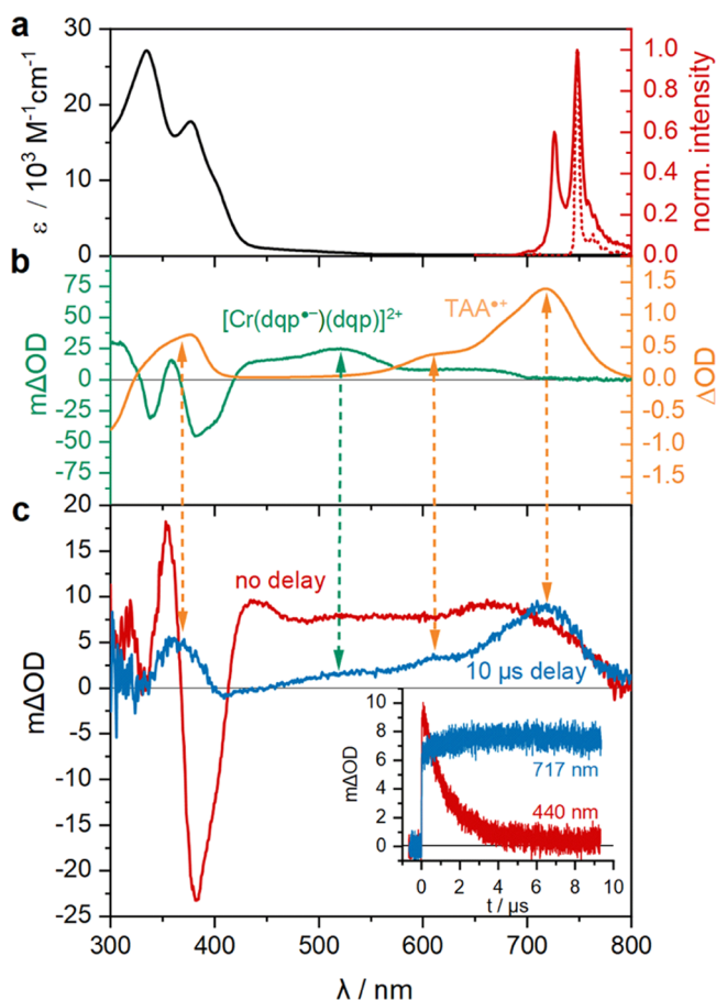
Figure 2. (a) UV-vis absorption (black) and emission spectra at 293 K in acetonitrile (solid red) and at 77 K in 1:1 (v/v) dimethyl sulfoxide (DMSO)/water (dotted red) of 35 \mu\text{M} [\text{Cr}(\text{dqp})_2](\text{PF}_6)_3 . The emission spectra were recorded following excitation at 410 nm. (b) Spectro-electrochemical UV-vis difference spectrum of 350 \mu\text{M} [\text{Cr}(\text{dqp})_2](\text{PF}_6)_3 in acetonitrile containing 0.1 M tetra- n -butylammonium hexafluorophosphate (TBAPF 6 ), obtained at an applied potential of -0.5 V vs SCE (green) along with the UV-vis difference spectrum of 400 \mu\text{M} TAA obtained in the same solvent by applying a potential of +0.8 V vs SCE (orange). The UV-vis spectra recorded prior to application of the potential served as a baseline in both cases. (c) Transient UV-vis absorption spectrum of 35 \mu\text{M} [\text{Cr}(\text{dqp})_2](\text{PF}_6)_3 and 100 \mu\text{M} TAA measured after excitation with 425 nm laser pulses of \sim 10 ns duration directly after the laser pulse (red) and after a delay of 10 \mu\text{s} (blue). Inset: Transient absorption decay at 440 nm, corresponding to the disappearance of {}^2\text{E}/{}^2\text{T}_1 -excited [\text{Cr}(\text{dqp})_2]^{3+} (red) and absorption growth at 717 nm, corresponding to TAA ^{\bullet+} formation (blue). All measurements were performed in dry and argon-saturated acetonitrile at 20 ^\circ\text{C} .
