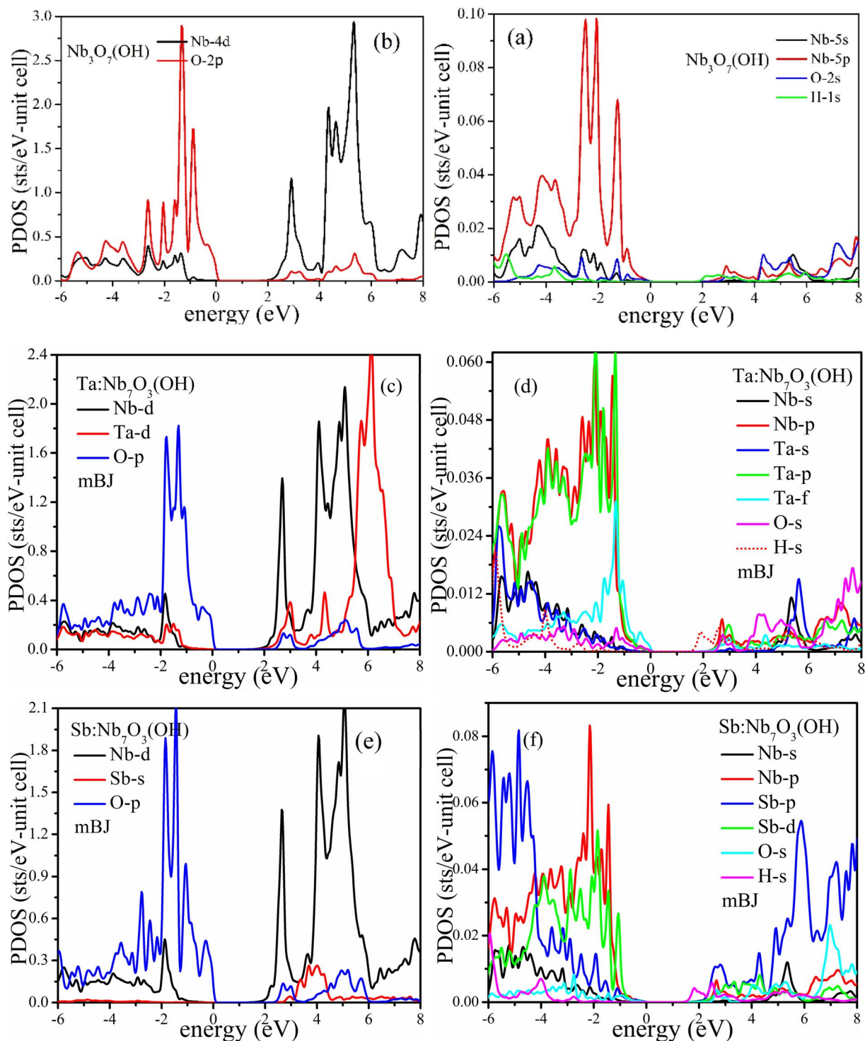
Fig. 3 Calculated partial density of states (PDOS) using Trans-Blaha modified Becke–Johnson approximation (TB-mBJ/TB-mBJ + SO). (a and b) PDOS of Nb 3 O 7 (OH). (c and d) PDOS of Ta:Nb 3 O 7 (OH). (e and f) PDOS of Sb:Nb 3 O 7 (OH).
