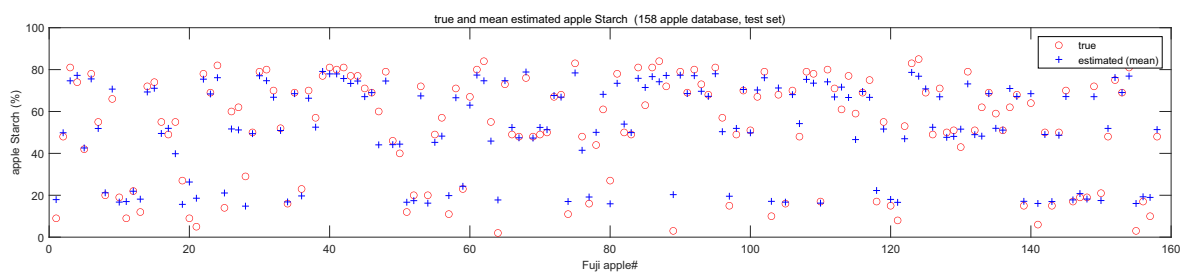
Figure 12. Scatter plot of actual and mean estimated value of 158 Fuji Apples in starch content (%) prediction at whole spectral 400–1000 nm range: test set.
