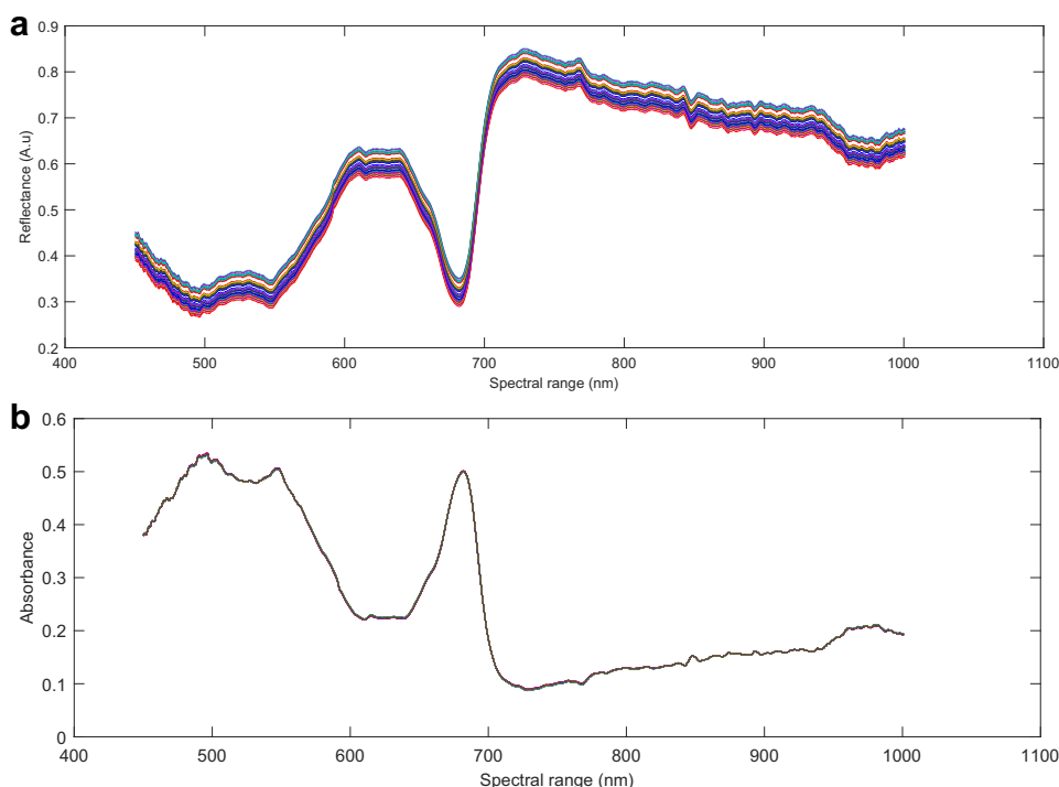
Figure 3. Spectral graphs of different apple input samples. (a) reflectance spectra of different samples; (b) pre-processed spectral absorbance spectra, as done in three steps: 1) conversion of reflectance to absorbance spectra with Eq. (1), 2) light scatter and baseline correction by MSC, and 3) smoothing of spectral peaks by median filtering.
