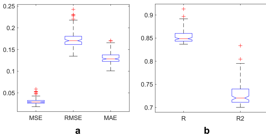
Figure 5. Boxplot diagram of different performance evaluation criteria: a) Error indices, b) Regression (R) and determination ( R^2 ) coefficients ANN-CA method in estimating firmness (kgf/cm) on the 400–1000 nm spectral data (test set).
