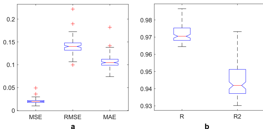
Figure 11. Boxplot diagram of different performance evaluation criteria: a) Error indices, b) Regression (R) and determination (R 2 ) coefficients, ANN-CA method in estimation of starch content (%) at whole spectral range of 400–1000 nm (test set).
