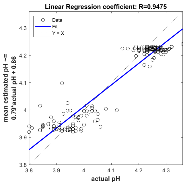
Figure 7. Linear regression plot between estimated (mean) and true acidity (pH) apple fruit values from spectral data of 400–1000 nm: test set.
