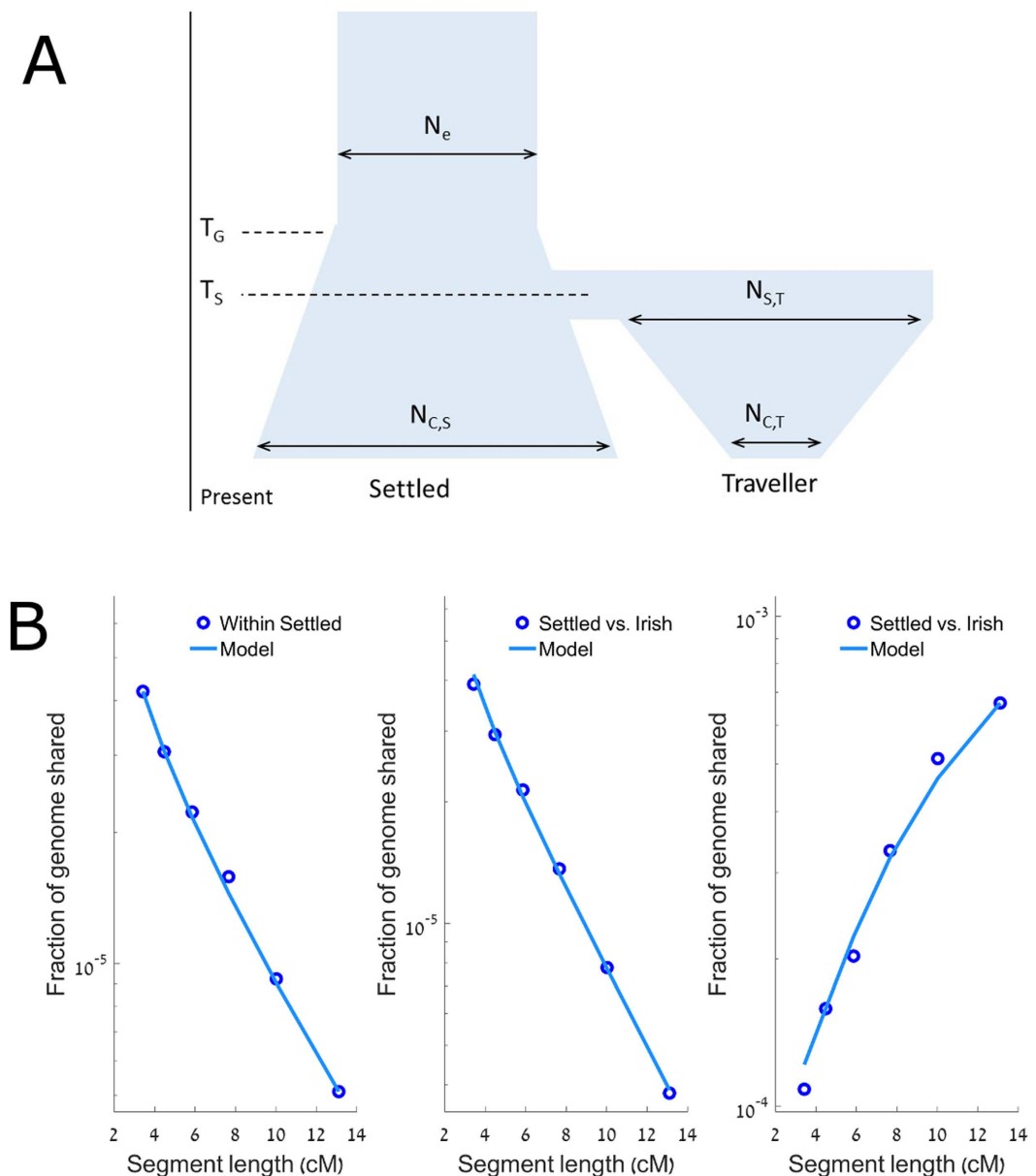
Figure 5. (A) The model used for demographic inference. The two populations were one ancestral population, with size N_e , T_G generations ago. At this point the ancestral population started to grow exponentially until T_S generations ago, where the ancestral Traveller and settled populations split from each other, with N_{S,T} being the initial starting population size of the Traveller population. The settled population experienced continued exponential growth until the present, with a population size of N_{C,S} . The Traveller population experienced a period of exponential contraction until the present, with a population of N_{C,T} . (B) The proportion of the genome in IBD segments vs the IBD segments length. The total genome size and the sum of segment lengths were computed in cM. Left: sharing between pairs of settled Irish; middle: sharing between pairs of one settled and one Traveller individuals; right: sharing between pairs of Traveller Irish. Each data point is located at the harmonic mean of the boundaries of the length interval it represents.
