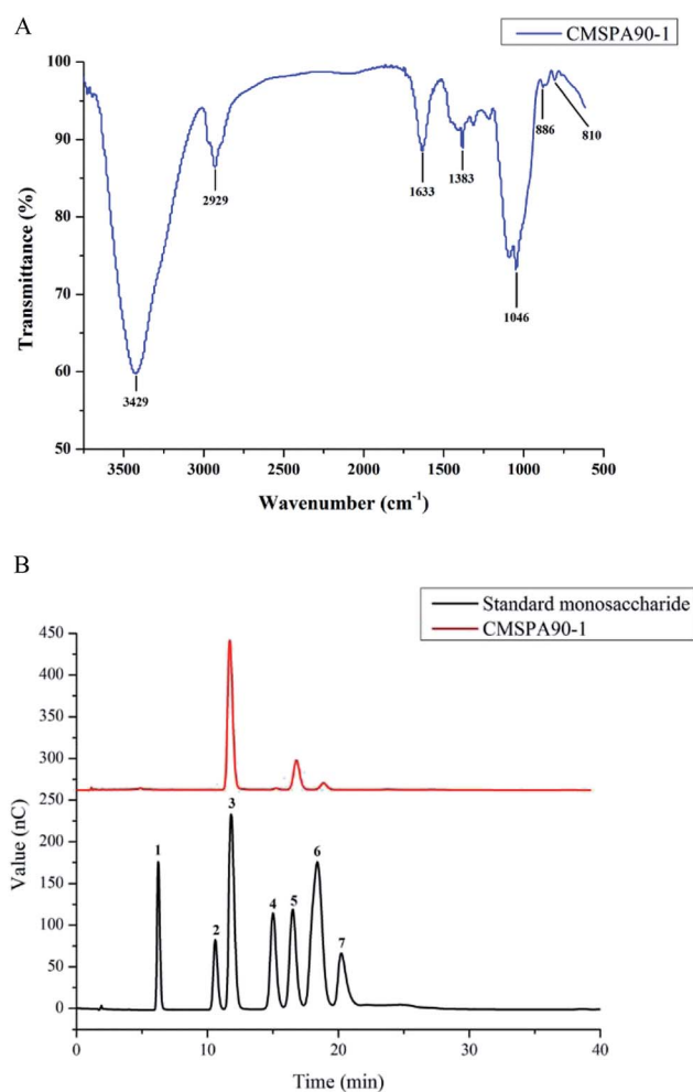
Fig. 2 FT-IR spectrum of CMSPA90-1 (A), HPAEC of standard monosaccharides and CMSPA90-1 peaks: (1) fucose, (2) rhamnose, (3) arabinose, (4) galactose, (5) glucose, (6) mannose, (7) fructose (B).
