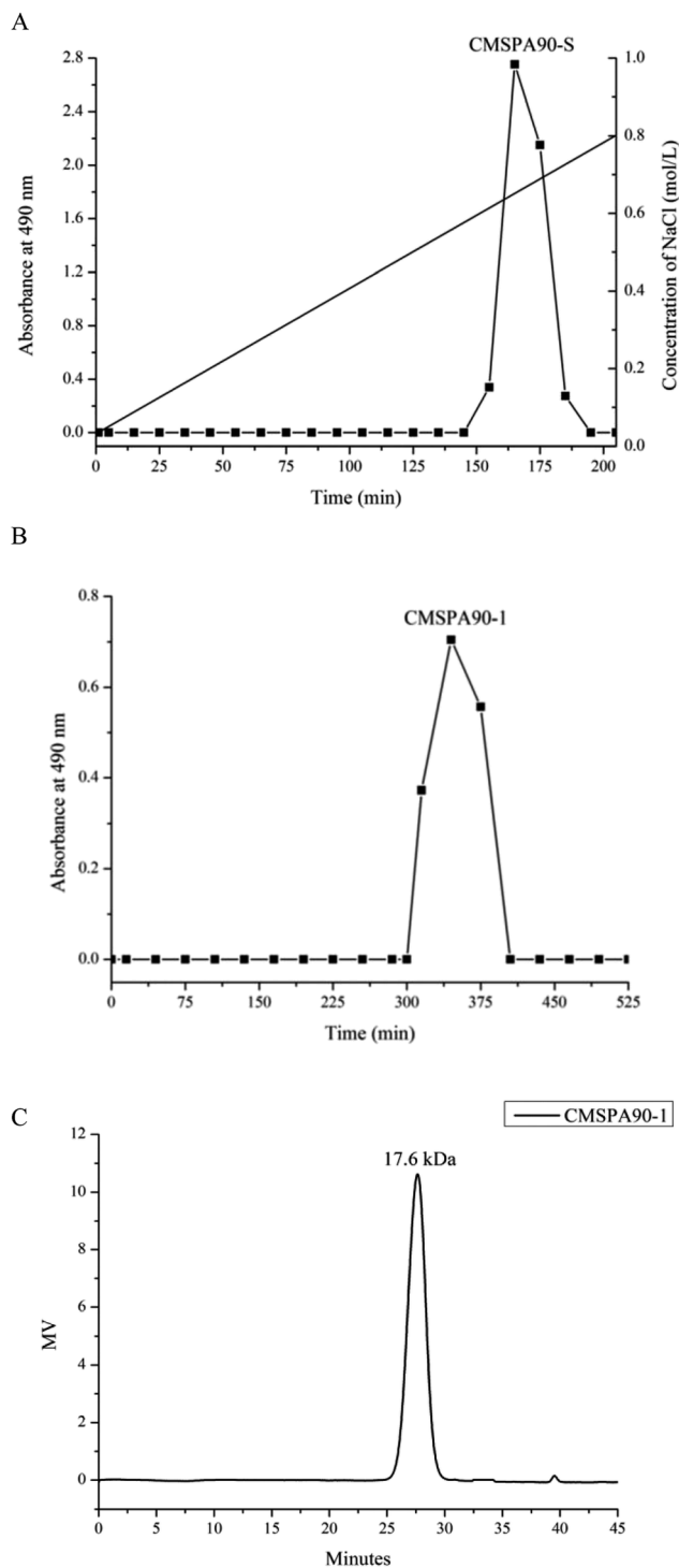
Fig. 1 Chromatography of CMSPA90 from bergamot by DEAE-sepharose fast flow chromatography (A), chromatography of CMSPA90-1 by sephadex G-75 (B), and HPGPC of CMSPA90-1 (C).
