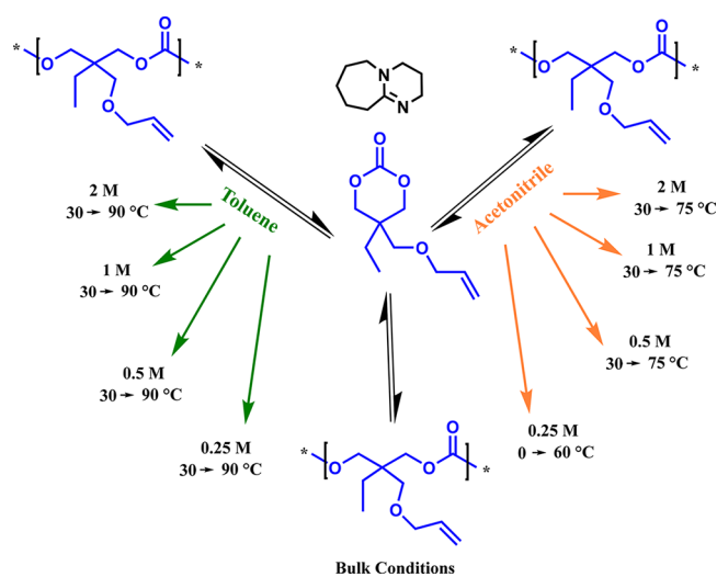
Scheme 2. Polymerization of AOMECA in PhMe and in MeCN with 5 mol % DBU (Relative to the Initial Monomer Concentration) as Catalyst Using Different Initial Monomer Concentrations and Polymerization Temperatures: Evaluation of the Equilibrium Conversion
