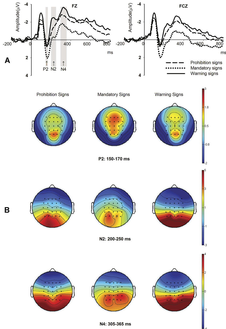
Figure 3 Event-related potentials (ERPs) results. (A) The grand averaged waveforms in the frontal and fronto-central sites; (B) The topographic maps of P2, N2 and N4 for different types of safety signs. P2 is the second positive component of ERPs; N2 is the second negative component of ERPs; N4 is a negative component of ERPs observed at around 400ms. FZ is a frontal midline scalp electrode and FCZ is a fronto-central midline scalp electrode.
