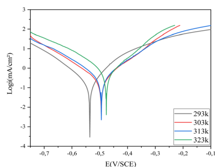
Fig. 6 Polarisation curves for Blank at different temperatures.
