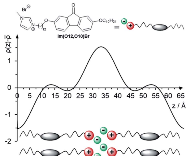
Fig. 15 Electron density profile of \text{Im}(\text{O12}, \text{O10})\text{Br} in the \text{SmA} phase at 167^\circ\text{C} indicating a bilayer structure and its suggested packing model.
