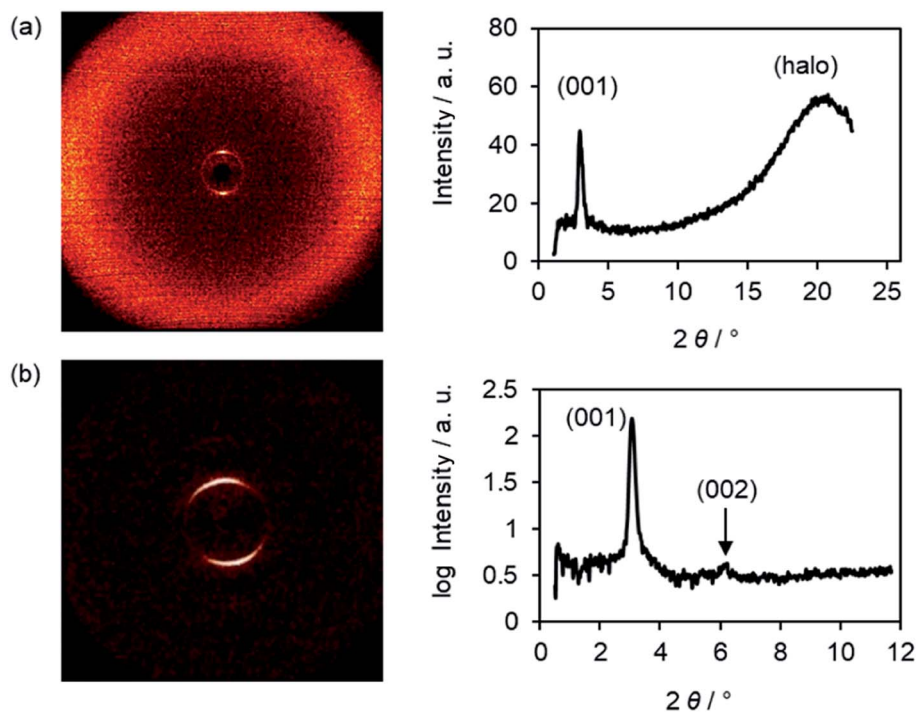
Fig. 2 (a) Wide-angle scattering (WAXS) and (b) small-angle scattering (SAXS) profile and the corresponding diffraction pattern of Br(O6,O8) at 45 \text{ }^\circ\text{C} .
