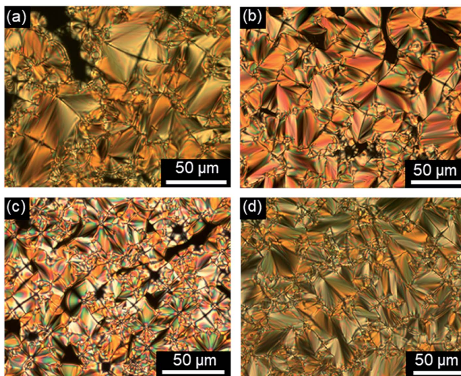
Fig. 1 Focal-conic fan textures as seen between crossed polarizers upon cooling from the isotropic liquid (cooling rate 5 \text{ K min}^{-1} , magnification \times 200 ). (a) Br(O4,O12) at 65 \text{ }^\circ\text{C} , (b) Br(O6,O12) at 71 \text{ }^\circ\text{C} , (c) Br(O8,S12) at 61 \text{ }^\circ\text{C} , and (d) Br(O10,O12) at 70 \text{ }^\circ\text{C} .
