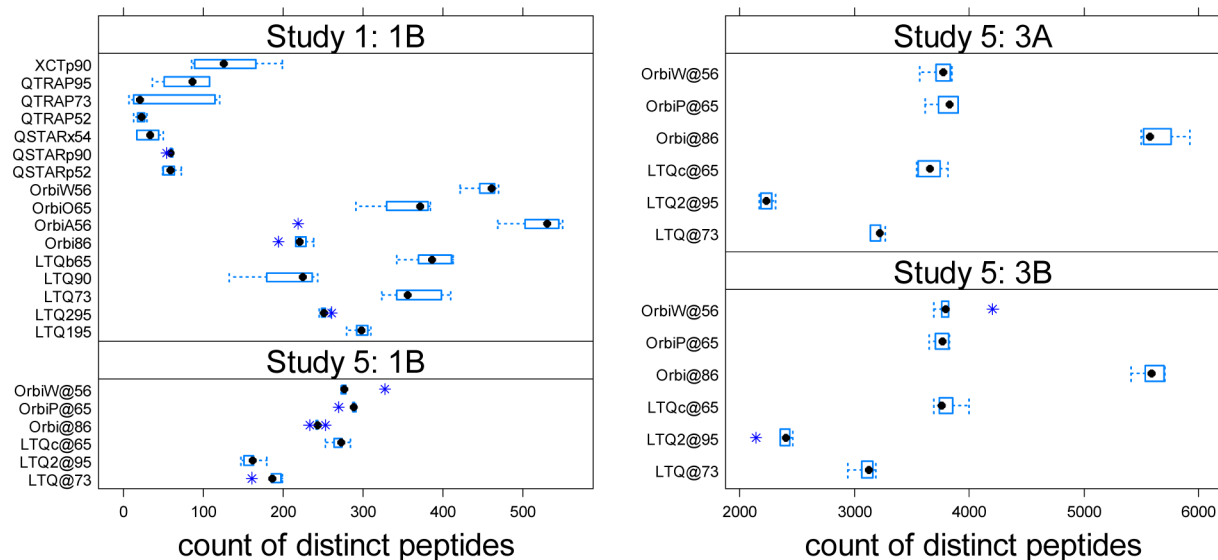
Figure 6. Numbers of peptides vs type of mass spectrometers employed in Study 1. The number of distinct peptides identified in each experiment bore a clear relationship to the type of instrument employed. While in each case instrument vendor libraries performed operations such as charge state determination and peak picking, the peak lists for identification may not have been optimal for a variety of reasons. For this informatics workflow in Study 1 (the upper panel on the left), the Orbitrap and LTQ-class instruments from Thermo identified a greater diversity of peptides than did the instruments from other manufacturers. Study 5 results (Sample 1B, the lower panel on the left; Sample 3A, the upper panel on the right; Sample 3B, the lower panel on the right) show that the Orbitrap has a larger number of peptides identified than LTQ. Orbi@86 yielded very high sensitivity for samples 3A and 3B, with OrbiP@65, OrbiW@56, and LTQc@65 trailing behind but still yielding more diverse peptide collections than the other LTQs.
