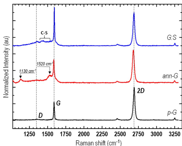
Fig. 3 Raman spectra of sulfurized single-layer graphene (G : S) on SiO 2 /Si (blue line) in comparison with the pristine graphene (p-G) single-layer (black line) before and after annealing (ann-G) at 230 °C (red line).
