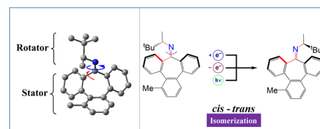
Fig. 1 (a) Schematic of the rotary cycle of the N -alkyl imine isomers. (b) The key geometric parameters \theta_{CCNC} and \theta_{CCCN} used in this work.
