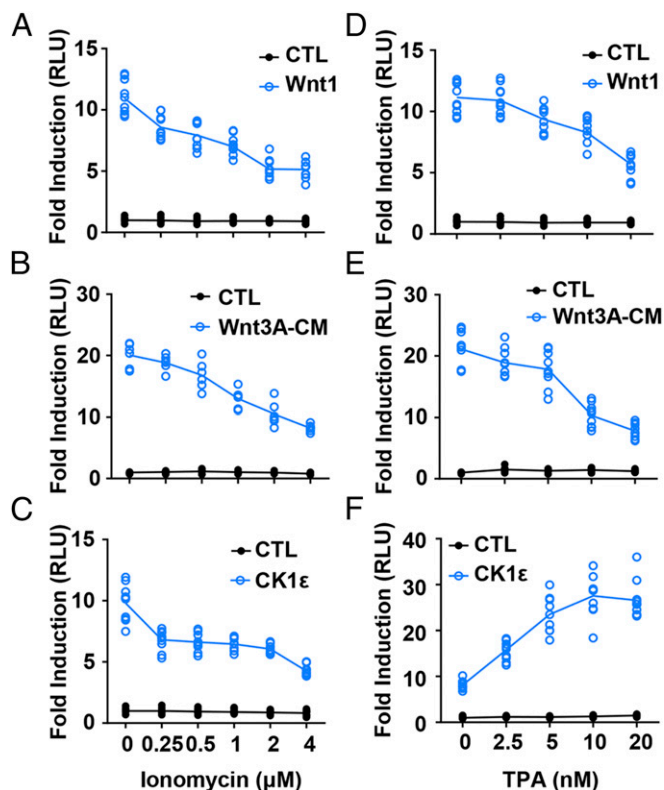
Fig. 1. TPA enhances Wnt/ \beta -catenin signaling activated by CK1 \epsilon . (A) A SuperTopFlash reporter gene was transfected into HEK293T cells together with empty vector or Wnt1 expression plasmid. The transfected cells were treated with vehicle or the indicated concentrations of ionomycin before being assayed for luciferase activity. (B) The SuperTopFlash reporter gene was transfected into HEK293T cells, after which the cells were treated with control or Wnt3A-CM. The cells were treated with vehicle or increasing concentrations of ionomycin as indicated. (C) HEK293T cells were transfected with the SuperTopFlash reporter gene and empty vector or an expression plasmid for CK1 \epsilon . The cells were incubated with vehicle or increasing concentrations of ionomycin as indicated. (D) Similar to A except that the indicated concentrations of TPA were used. (E) Similar to B except that the indicated concentrations of TPA were used. (F) Similar to C except that the indicated concentrations of TPA were used. The luciferase values were normalized to \beta -gal activities. Results are expressed as fold induction compared with empty vector control. The results were the average from at least three independent experiments done by duplicates, n \geq 6 .
