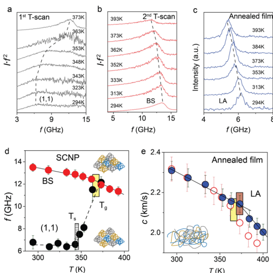
Figure 4. BLS spectra of SCNPs in three different morphologies. Evolution of the reduced BLS spectra, I f^2 vs f , with temperature ( T ) for (a) the as-prepared SCNPs sample (1st T-scan) and (b) the coalescent SCNPs obtained after quenching of the as-prepared SCNP sample in (a) from 373 K (2nd T-scan), (c) BLS spectra ( I vs f ) of the transparent annealed PS film obtained after annealing under vacuum at 423 K for 24 h of the coalescent SCNP film in (b). The dashed lines indicate the variation of the frequency f_{(1,1)} of (1,1) mode in (a) and longitudinal phonon f at scattering angle 180^\circ in (b) and at 90^\circ in (c) with T . The dashed lines in (a–c) are guides to the eye. (d) T dependence of f_{(1,1)} (black solid symbols) in the as-prepared SCNPs sample in (a) and the frequency of LA (red solid symbols) in the coalescent SCNPs sample in (b). The lower and upper insets indicate the schematics of the as-prepared SCNPs and the coalescent SCNPs. (e) T dependence of the longitudinal sound velocity, c , of the transparent annealed film (blue solid symbols) obtained from the BLS spectra in (c) and the coalescent SCNPs of the 2nd T-scan (open red symbols) obtained from the f in (d). The solid lines denote the linear c(T) below and above T_g . The patterned and shaded areas denote the softening temperature T_s in the 1st T-scan and the glass transition temperature T_g for the three samples, respectively.
