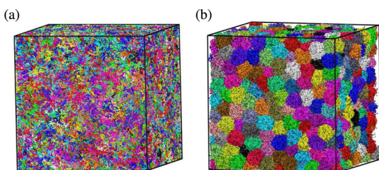
Figure 5. Snapshots of the two different polymer melts of an equilibrated system (a) and a melt of individually collapsed, disentangled chains (b) of the very same length. Each system contains 1000 chains of chain length N = 1000 with the monomer density \rho = 0.85\sigma^{-3} .
