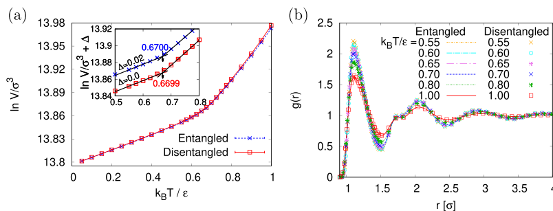
Figure 6. MD simulations: (a) logarithm of volume of the system, \ln V/\sigma^3 , plotted vs temperature k_B T/\epsilon . (b) Radial nonbonded monomer–monomer distribution function g(r) for disentangled and entangled polymer melts. Several values of T are chosen, as indicated. In (a), the two linear lines give the best fit of our data along the liquid branch ( a_{\text{liquid}}^{(\text{disent})} \approx 13.6681 , \alpha_{\text{liquid}}^{(\text{disent})} \approx 0.2981k_B/\epsilon ), ( a_{\text{liquid}}^{(\text{ent})} \approx 13.6733 , \alpha_{\text{liquid}}^{(\text{ent})} \approx 0.2896k_B/\epsilon ) and the glass branch ( a_{\text{glass}}^{(\text{disent})} \approx 13.7784 , \alpha_{\text{glass}}^{(\text{disent})} \approx 0.1333k_B/\epsilon ), ( a_{\text{glass}}^{(\text{ent})} \approx 13.7776 , \alpha_{\text{glass}}^{(\text{ent})} \approx 0.1339k_B/\epsilon ) for disentangled and entangled polymer melts, respectively. The error bars of the data are within the size of symbols. In the inset data for the same quench rate but a much smaller T range are given for comparison. Data for the entangled polymer melt are shifted by a constant \Delta = 0.02 for a better illustration. Confined to that small interval the shift in T_g diminishes.
