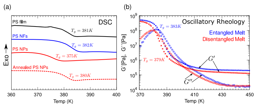
Figure 3. Comparison of the glass transition temperature T_g of entangled and disentangled PS: (a) DSC experiments: PS NPs, PS NFs, and PS film. PS NPs and NFs were prepared by electrospinning of PS in DMF solution at concentrations C = 0.2 wt % and C = 2.3 wt % using the process parameters: distance d = 20 cm and infuse-rate \nu = 1.5 mL/h and applied voltage V = 15 kV. PS film was prepared by hot-pressing bulk PS at temperature T = 433 K under a load of L = 20 kN. (b) Rheological experiment: temperature sweep at frequency f = 10 rad/s was used.
