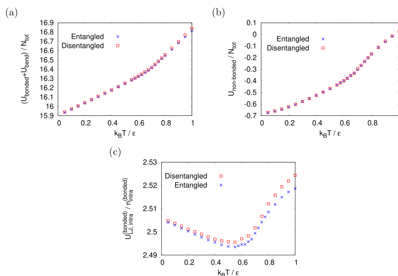
Figure 7. Temperature dependence of the average bonded and bending (a) and nonbonded (b) potential energies per monomer and repulsive part of the bonded potential energy per monomer pairs (c).
