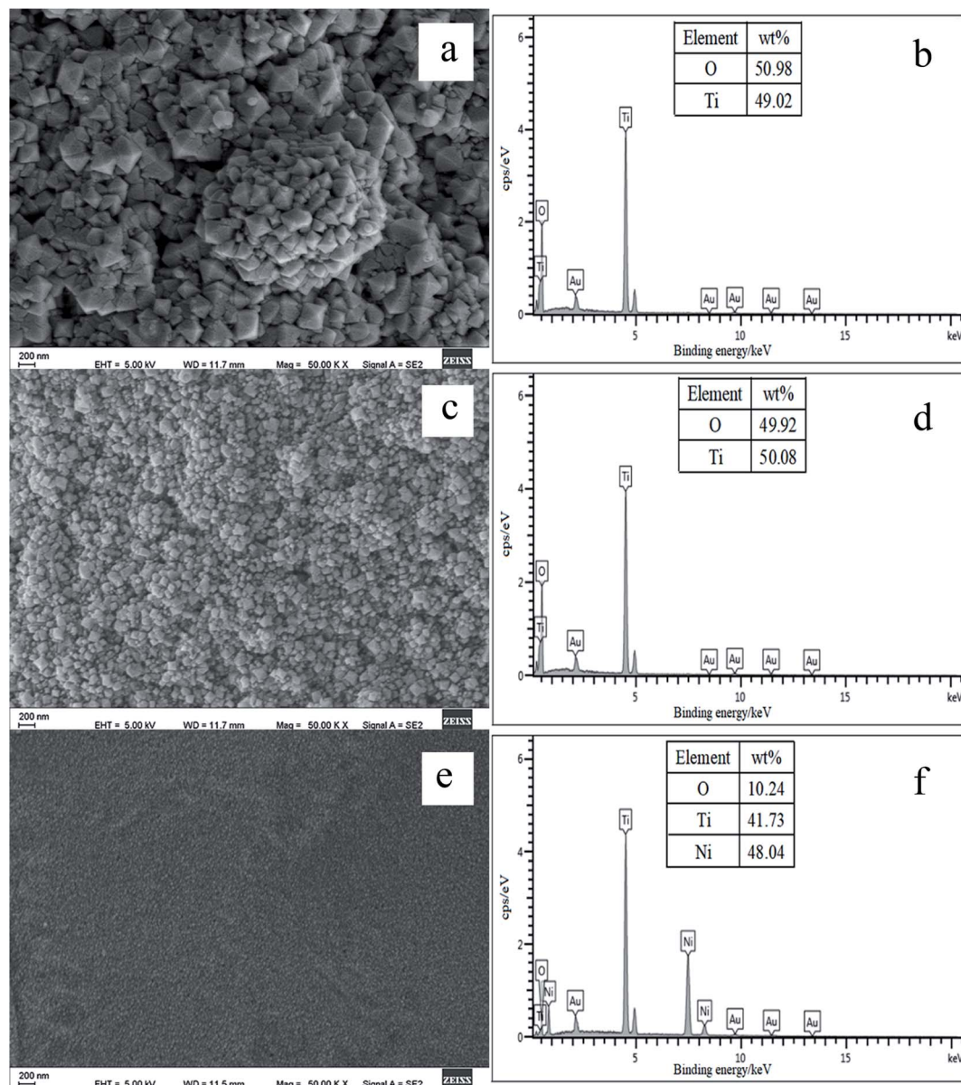
Fig. 1 Surface SEM images and EDX spectra of the oxide coatings grown on the pretreated NiTi wire by hydrothermal reaction in HCl solution (a and b), \text{HNO}_3 solution (c and d) and glacial acetic acid (e and f) at 150^\circ\text{C} for 12 h.
