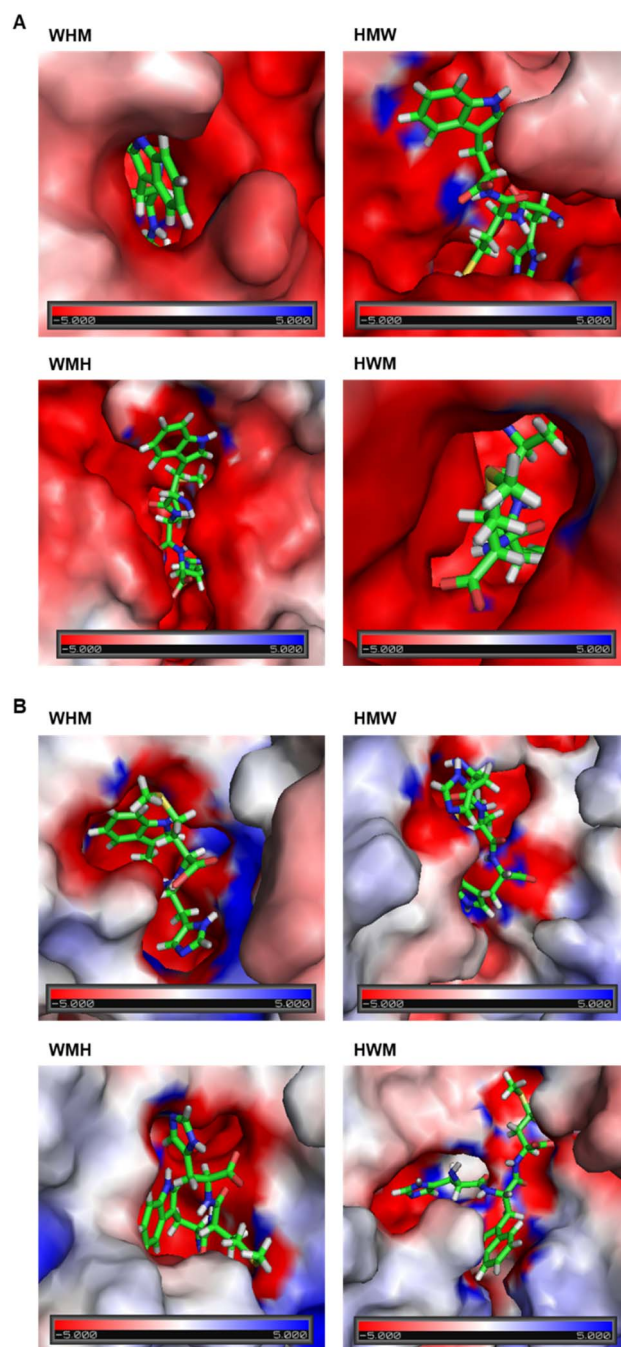
Fig. 4 Electrostatic potential maps of AChE (in A) and BACE-1 (in B) binding pockets in complexes with tripeptides. Blue regions represent areas of positive electrostatic potential, while red regions indicate negative electrostatic potential. The intensity of the electrostatic potential reflects the strength of charge distribution within the active site.
