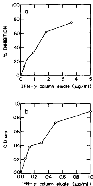
FIGURE 4. (a) Inhibition of 125 I-rIFN- \gamma binding in sRIA by ligand (IFN- \gamma ) affinity-purified urinary proteins. Maximal binding with 125 I-rIFN- \gamma alone was 4,300 cpm. Background binding (200 cpm) was determined in the presence of excess unlabeled rIFN- \gamma and was subtracted from all readings. Immunoaffinity-purified IFN- \gamma -R from human placenta (8) (8 \mu g/ml) was used as a positive control and gave 80% inhibition. Ligand (IL-6) affinity-purified urinary protein (10 \mu g/ml) was used as a negative control and gave only 10% inhibition. (b) Characterization of IFN- \gamma binding proteins as receptors by a double-antibody ELISA. Immunoaffinity-purified IFN- \gamma -R from human placenta (8) (0.5 \mu g/ml) was used as a positive control and gave 0.45 OD 600 . Ligand (IL-6) affinity-purified urinary proteins (0.5 \mu g/ml) were used as a negative control and gave 0.06 OD 600 .
