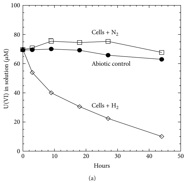
FIGURE 4: Hydrogen-driven reduction of U(VI) (a) and Fe(III) (b) by Clostridium sp. BCl.
