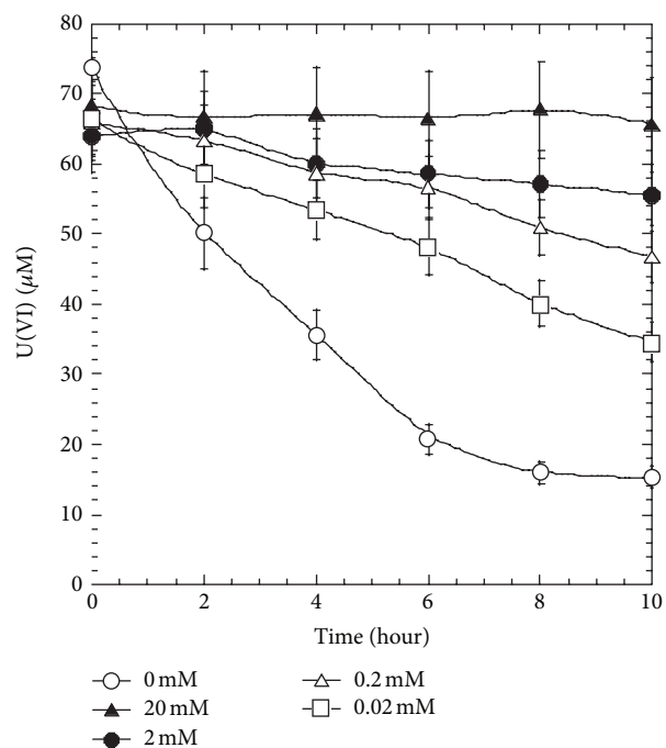
FIGURE 5: Effect of addition of Copper(II) on uranium reduction by Clostridium sp. BCl.
