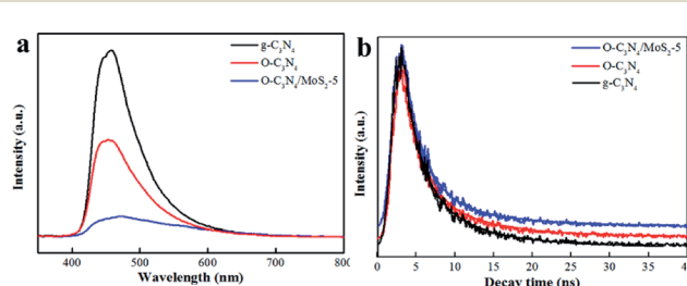
Fig. 6 (a) PL spectra and (b) time-resolved photoluminescence spectra of samples with an excitation wavelength of 330 nm.
