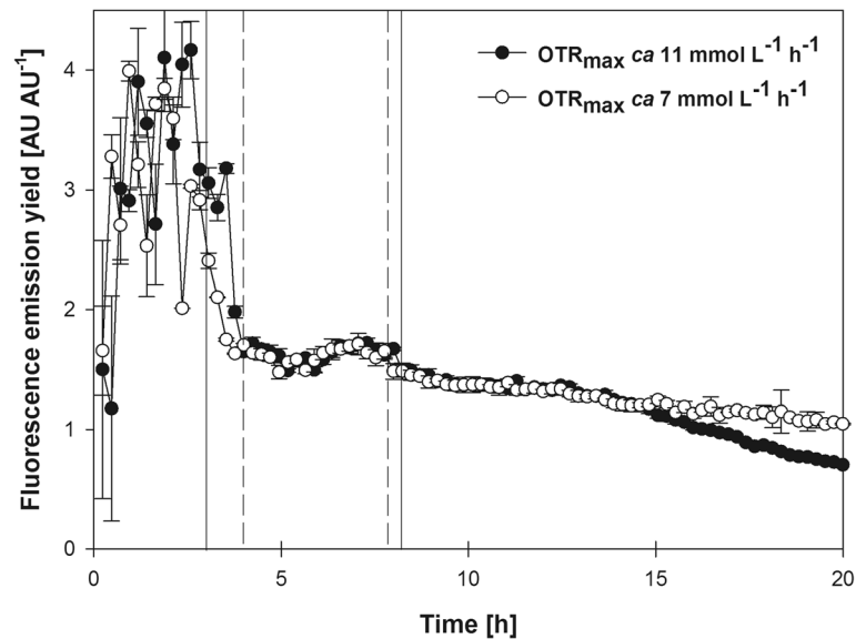
Fig. 2 Fluorescence emission yield during oxygen-limited cultures of E. coli expressing FbFP under control of P_{k_{OT}} . The vertical solid (for OTR_{max} ca. 7 \text{ mmol L}^{-1} \text{ h}^{-1} ) and dashed (for OTR_{max} ca. 11 \text{ mmol L}^{-1} \text{ h}^{-1} ) lines indicate the beginning (lines to the left) and end (lines to the right) of the oxygen-limited phases. Fluorescence yields were calculated by dividing the FbFP fluorescence intensity signal by the scattered light intensity signal at every time-point. Vertical lines show the standard deviation ( n = 3 ) of average values
