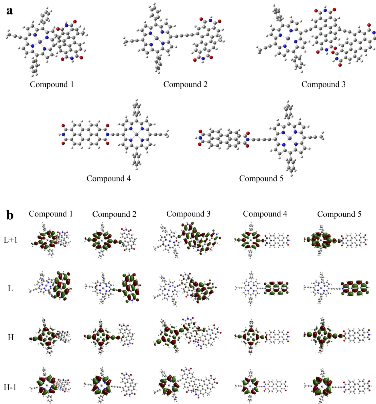
Fig. 8 (a) Optimized ground-state structures of compounds 1–5 and (b) illustrations of the molecular orbitals of compounds 1–5.
