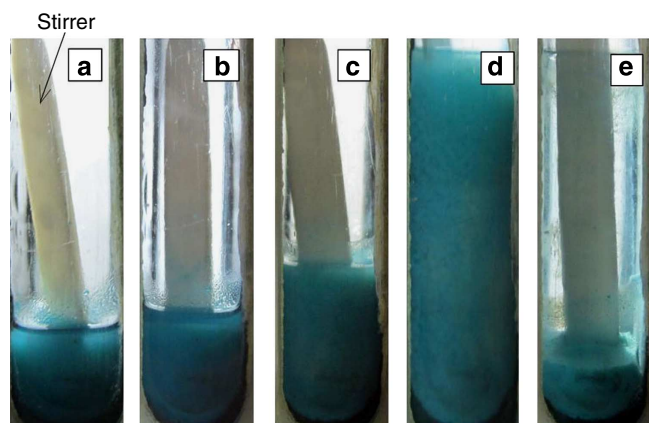
Figure 1 | Photographs of MOF synthesis in CO 2 -expanded DMF. (a) In pure DMF; (b) 2.0; (c) 4.5; (d) 6.6 MPa. (e) Phase separation in reaction system at 6.6 MPa after reaction for 3 h.
