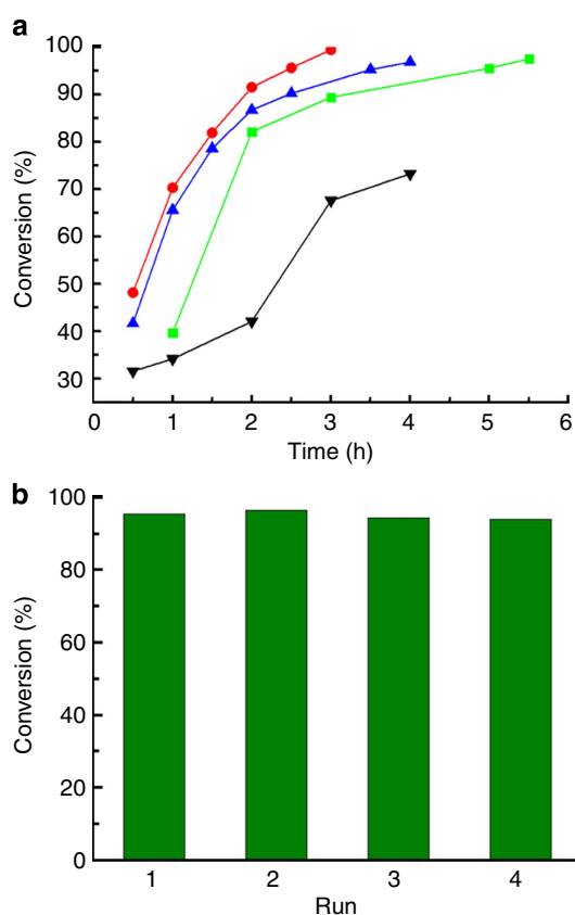
Figure 5 | Oxidation of benzyl alcohol using Cu 3 (BTC) 2 with oxygen.
