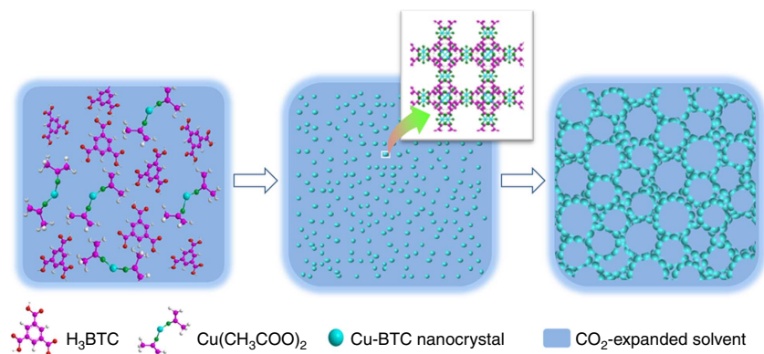
Figure 4 | Schematic illustration for mesocellular MOF formation. The Cu 2+ ions react with the deprotonated BTC 3- in the CXL and the nanosized framework building blocks are produced. Then the MOF building blocks assemble to form the mesocellular MOFs with large mesopores and thin mesopore walls.
