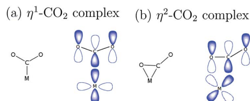
Fig. 1 (a) \eta^1 and (b) \eta^2 bonding scheme of M-CO 2 complexes.
