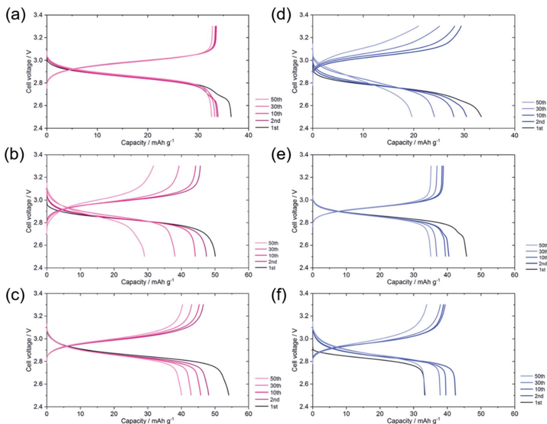
Fig. 5 Charge and discharge curves for \text{Li}|\text{Li}(\text{G3})|\text{TFSA}||\text{Li}(\text{G3})|\text{FeX} : \text{Li}(\text{G3})|\text{TFSA} = 5 : 95 C cell; (a) \text{X} = \text{Br}_4 , (b) \text{X} = \text{Cl}_3\text{Br} , (c) \text{X} = \text{Cl}_4 , and \text{Li}|\text{Li}(\text{G3Bu})|\text{TFSA}||\text{Li}(\text{G3Bu})|\text{FeX} : \text{Li}(\text{G3Bu})|\text{TFSA} = 5 : 95 C cell; (d) \text{X} = \text{Br}_4 , (e) \text{X} = \text{Cl}_3\text{Br} , (f) \text{X} = \text{Cl}_4 , at 30^\circ\text{C} at a rate of 0.2\text{C} .
