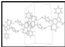
Fig. 2. The packing diagram of the title compound viewed along the a axis.
