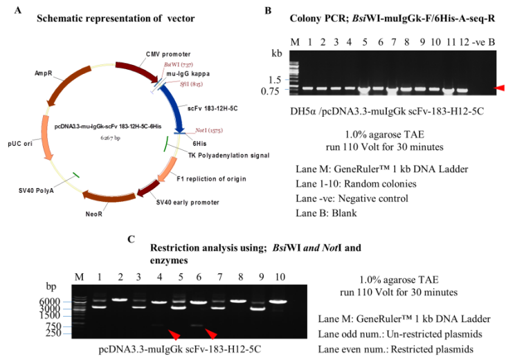
Figure 2. Engineering and verification of pCDNA3.3-muIgGk-scFv 183-H12-5C vector. Schematic representation of expression vector pCDNA3.3-muIgGk-scFv 183-H12-5C (A). Colony PCR used BsiWI -mulgGk-F/6His-A-seq-R primers; Presence of ~860 bp band in most of the clones suggests the presence of mu-IgGk-scFv 183-H12-5C in pCDNA3.3-muIgGk-scFv 183-H12-5C plasmid vector (B). Restriction analysis of pCDNA3.3-muIgGk-scFv 183-H12-5C with BsiWI/NotI (5.4 kb vector backbone + 855 bp insert) (C).
