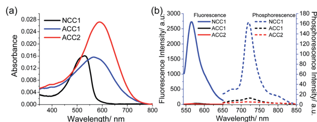
Fig. 1 (a) UV-vis absorption spectra of 1 \mu\text{M} NCC1 , ACC1 and ACC2 in PBS 7.4 and (b) fluorescence emission spectra of 1 \mu\text{M} NCC1 , ACC1 and ACC2 in PBS at 530 nm excitation (solid line) and phosphorescence spectra of 5 mM NCC1 , ACC1 and ACC2 in EtOH at -196^\circ\text{C} (dotted line).
