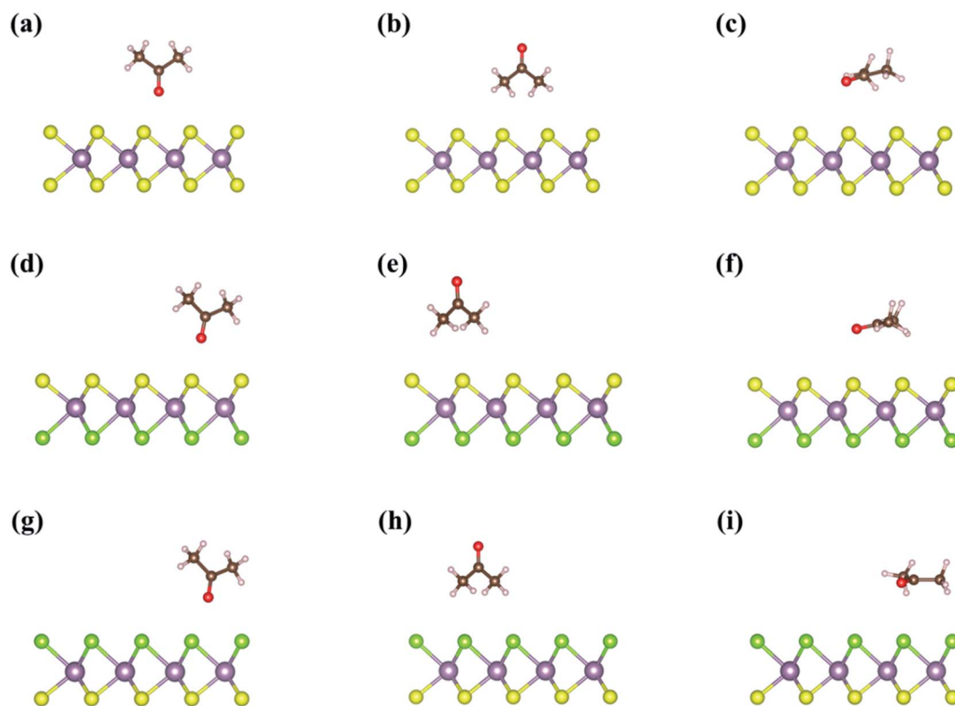
Fig. 2 Optimized adsorption structures of acetone on the TMDs monolayers without the external electric fields: (a) \text{Ace}_{v1} , (b) \text{Ace}_{v2} , and (c) \text{Ace}_h , on \text{MoS}_2 ; (d) \text{Ace}_{v1} , (e) \text{Ace}_{v2} , and (f) \text{Ace}_h , on S-layer of the Janus \text{MoSSe} ; (g) \text{Ace}_{v1} , (h) \text{Ace}_{v2} and (i) \text{Ace}_h , on Se-layer of the Janus \text{MoSSe} . Purple, yellow, and green spheres represent Mo, S, and Se atoms, respectively, while brown, red, and light pink balls are C, O, and H atoms, respectively.
