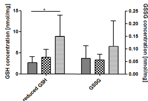
Figure 2: Reduced GSH and GSSG during aging rat liver cytosolic (A) and mitochondria-enriched (B) fractions as determined by photometric analysis. Values are mean \pm SD of 6-8 rats per age group. Significant differences (determined by One-way ANOVA) to the young group (* p < 0.05 , ** p < 0.01 ) are indicated.
