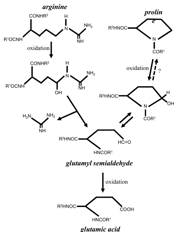
Figure 1. Iron-catalyzed oxidations of arginine and proline residues that result in the formation of glutamyl semialdehyde with a carbonyl group (Amici et al. , 1989).
