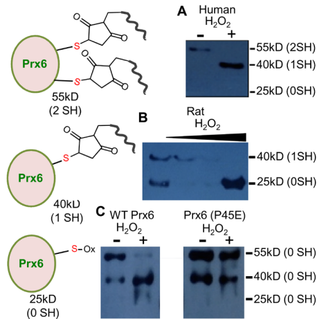
Figure 5. Proline 45 to glutamic acid conversion inhibits oxidation of active cysteine 47. Cultured human cells were treated with H_2O_2 (1 mM) for 15 min. Cellular proteins were precipitated with trichloroacetic acid and lysate samples were prepared for SulfoBiotics Protein Redox State Monitoring Kit Plus (Dojindo Molecular Technologies). Protein-SHifter that covalently binds to reduced protein thiols was added and samples were subjected to electrophoresis through a polyacrylamide gel. Each Protein SHifter causes \sim 15 kDa shift of the protein bands. After electrophoresis, the gel was exposed to UV irradiation to excise the Protein-SHifter Plus moiety, and then subjected to electrotransfer and Western blotting with the Prx6 antibody. In untreated cells, a 55 kDa band was primarily observed, indicating that two reduced cysteine residues in human Prx6 interacted with the SHifter. H_2O_2 treatment converted this to a 40 kDa band that is consistent with the Prx6 molecule with one cysteine oxidized. Human Prx6 contains two cysteine residues, one being the conserved catalytic cysteine 47 essential for its peroxidase activity and the other cysteine that is not conserved. (B) Cultured rat cells were treated with H_2O_2 and the same experiments were performed. Rat Prx6 contains only one cysteine that is the catalytic cysteine 47. Untreated rat cell lysates exhibited the 40 kDa band that is consistent with cysteine 47 being reduced. The treatment with H_2O_2 caused the disappearance of the 40 kDa band, suggesting that cysteine 47 is susceptible to oxidation. (C) Cells were infected with adenovirus expressing wild type (WT) Prx6 or Prx6 mutant with proline 45 replaced with glutamic acid (P45E) and treated with H_2O_2 , followed by Protein Redox State assay. Similarly to the results in Panel A , ectopically expressed wild type human Prx6 exhibited a 55 kDa band without H_2O_2 treatment and H_2O_2 formed a 40 kDa band. This oxidation of cysteine 47 does not occur in mutant Prx6 (P45E), revealing that converting proline 45 to glutamic acid inhibits the oxidation of catalytic cysteine 47 by H_2O_2 .
