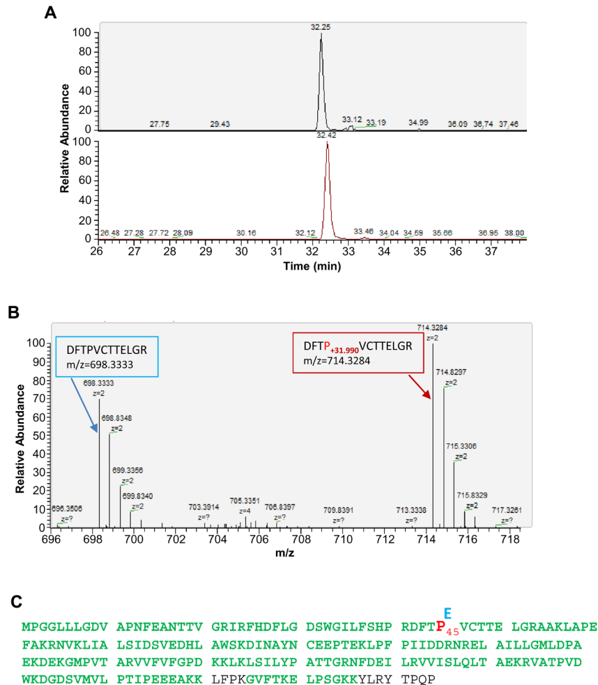
Figure 2. Identification of the conversion of the proline (P) residue at amino acid 45 into glutamic acid (E) in human peroxiredoxin 6 (Prx6). (A) Extracted ion chromatograms of Prx6 peptide (DFT P +31.990 VCTTELGR, +2 charge, m/z=714.33) (top) and its non-conversion counterpart (DFTPVCCTELGR, +2 charge, m/z=698.33) (bottom). Both peptides were eluted at the same retention time and are from affinity-enriched cultured human cell extract using the anti-Prx6 antibody. (B) High resolution MS spectra of the co-elution of peptides (DFTP +31.990 VCTTELGR, +2 charge, m/z=714.33) (right) and its non-conversion counterpart (DFTPVCCTELGR, +2 charge, m/z=698.33) (left). (C) Illustration of the identified proline 45 conversion into glutamic acid in cultured human cells (shown in bold red). Sequence areas containing amino acid residues shown in green are detected by LC-MS/MS analysis after trypsin digestion.
