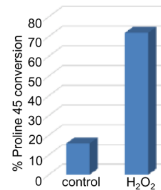
Figure 4. H 2 O 2 promotes proline 45 conversion within Prx6 protein in human cells. Cells were treated with H 2 O 2 (1 mM) for 10 min. Cell lysates were prepared and immunoprecipitated with the Prx6 antibody. Samples were subjected to MS/MS analysis. % of Prx6 with proline 45 conversion with the mass shift of + 31.990 Da increased from ~10% to ~70% after treating cells with H 2 O 2 for 10 min.
