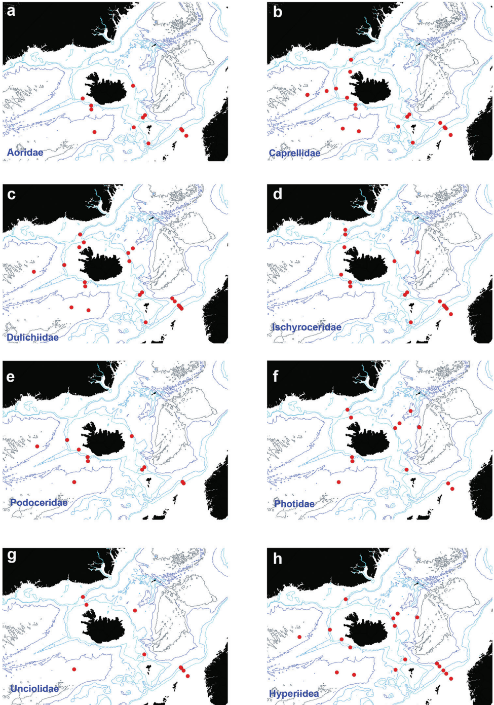
Figure 7. Distribution map for Corophiida a Aoridae b Caprellidae c Dulichiidae d Ischyroceridae e Podoceridae f Photidae g Uncioliidae h Hyperiidea, in sorted IceAGE EBS samples.
